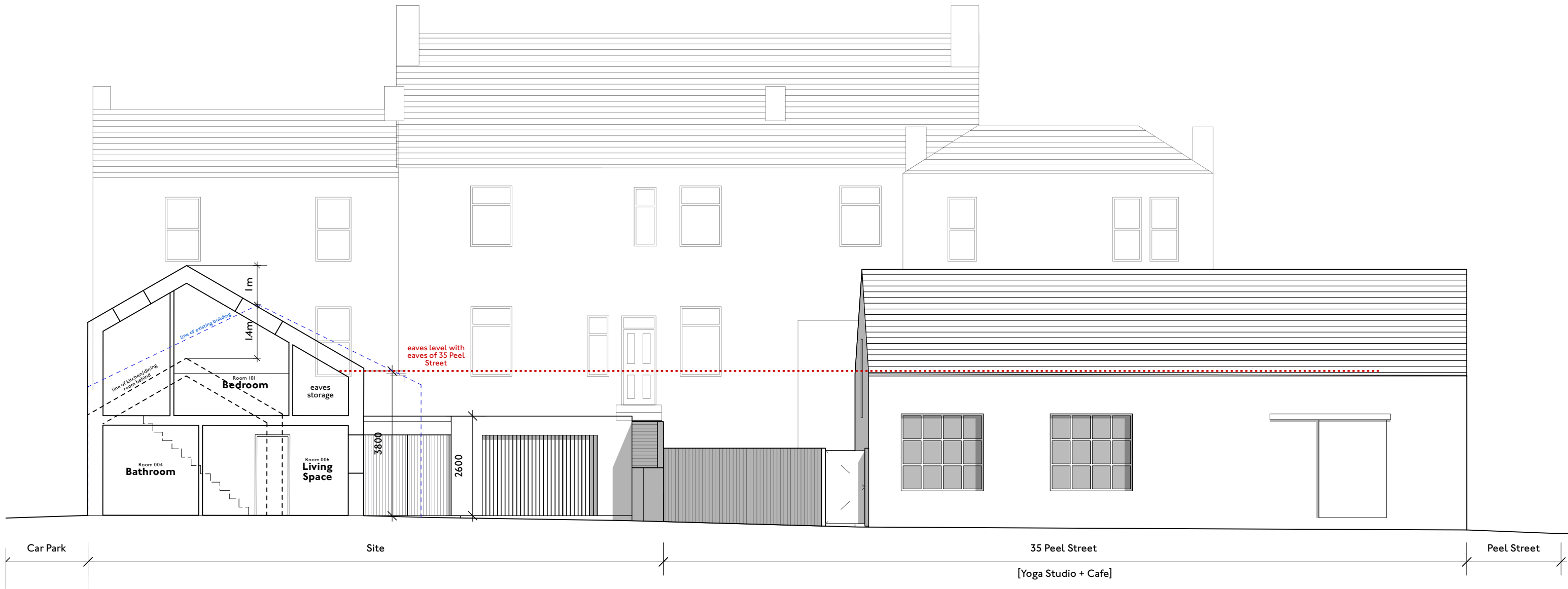
1 | 1:100 Section BB
