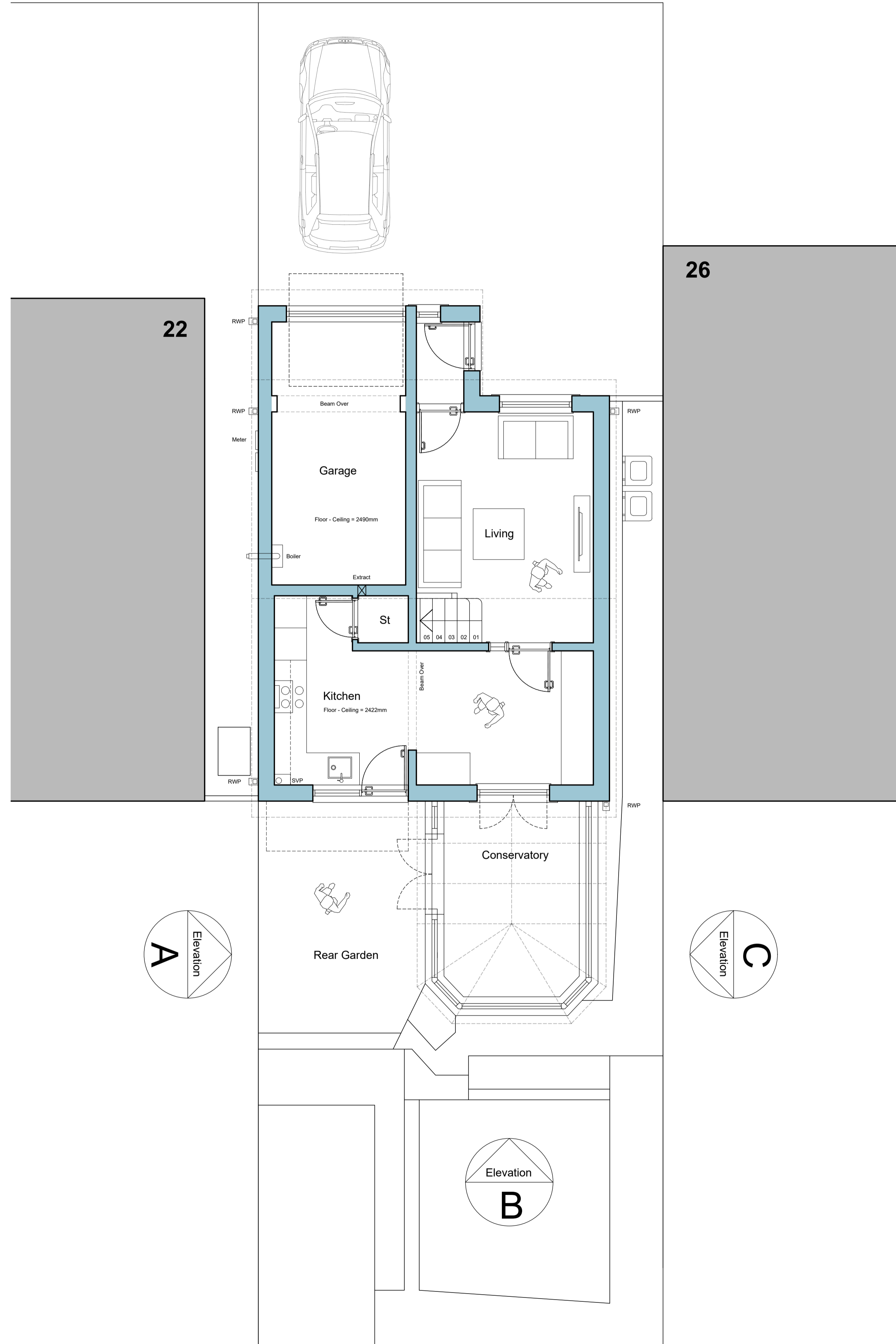
Existing Ground Floor Plan 1:50 @ A1
