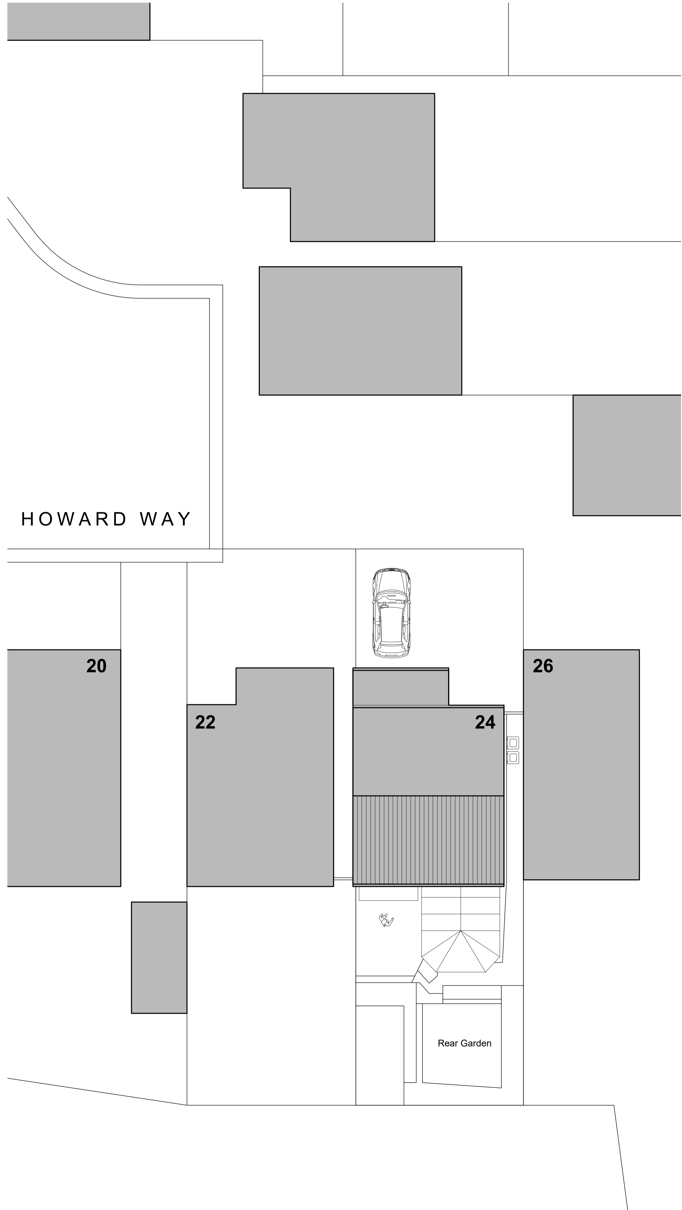
Existing Site Plan 1:100 @ A1
