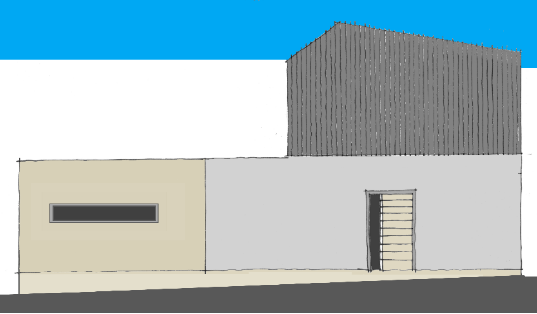
EAST ELEVATION - 1:100
