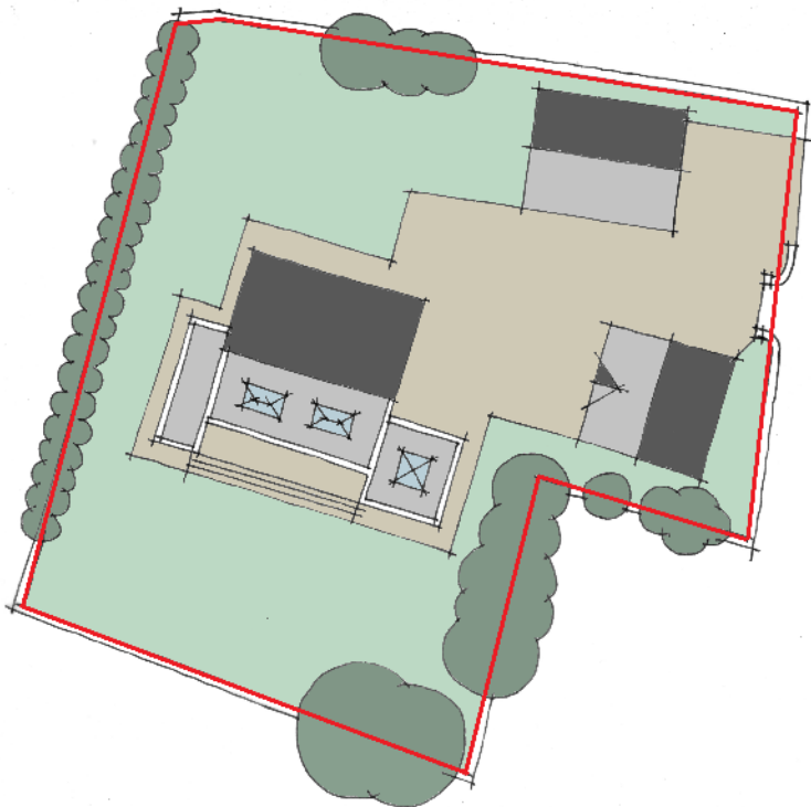
BLOCK PLAN - 1:500
