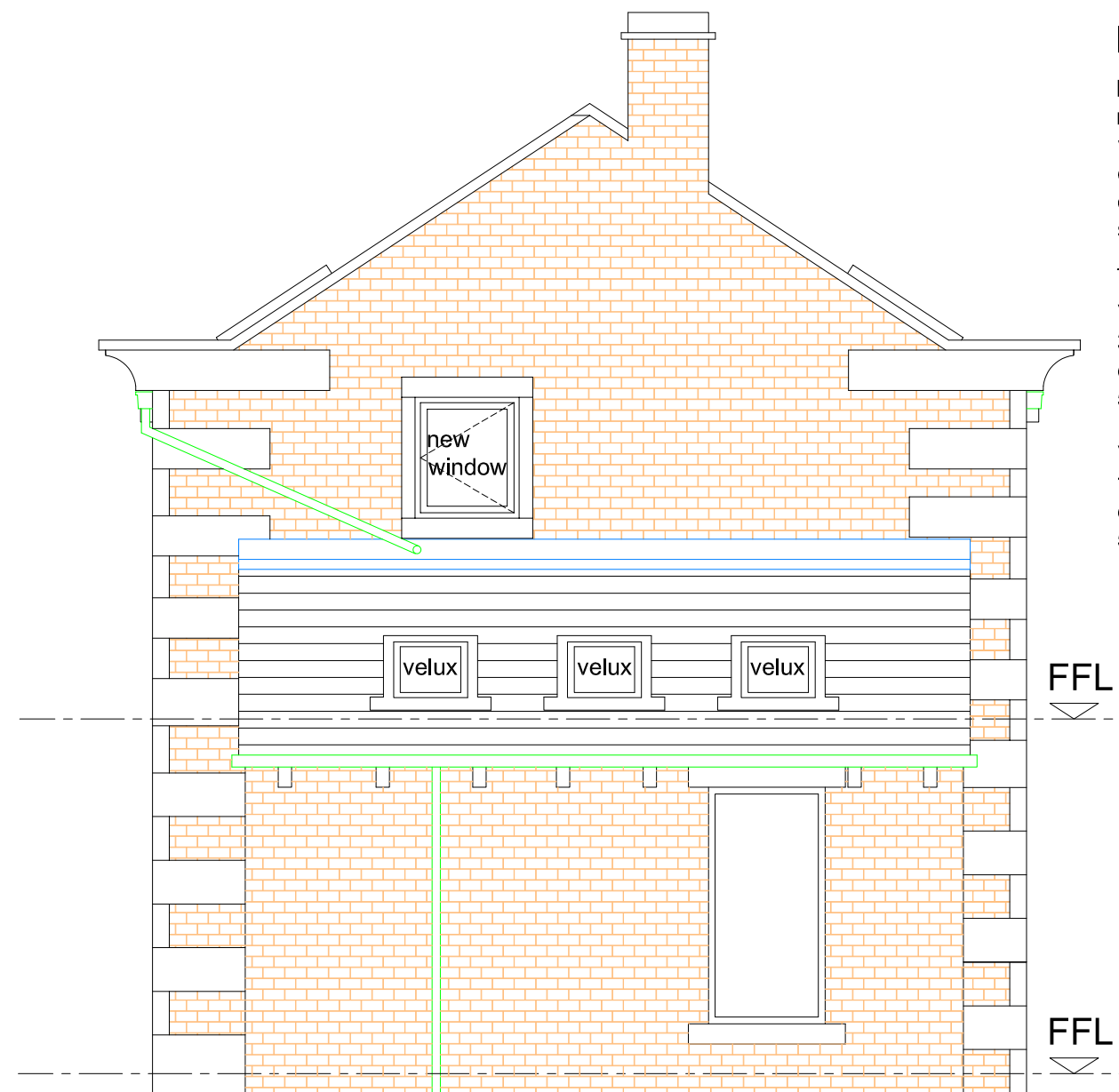
GABLE ELEVATION AS PROPOSED (NORTH) - 1:50
