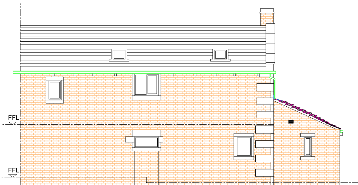
REAR ELEVATION AS EXISTING (EAST) - 1:100
