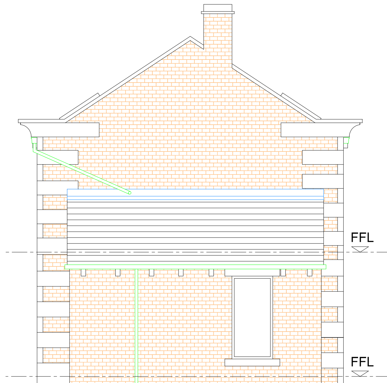
GABLE ELEVATION AS EXISTING (NORTH) - 1:50
