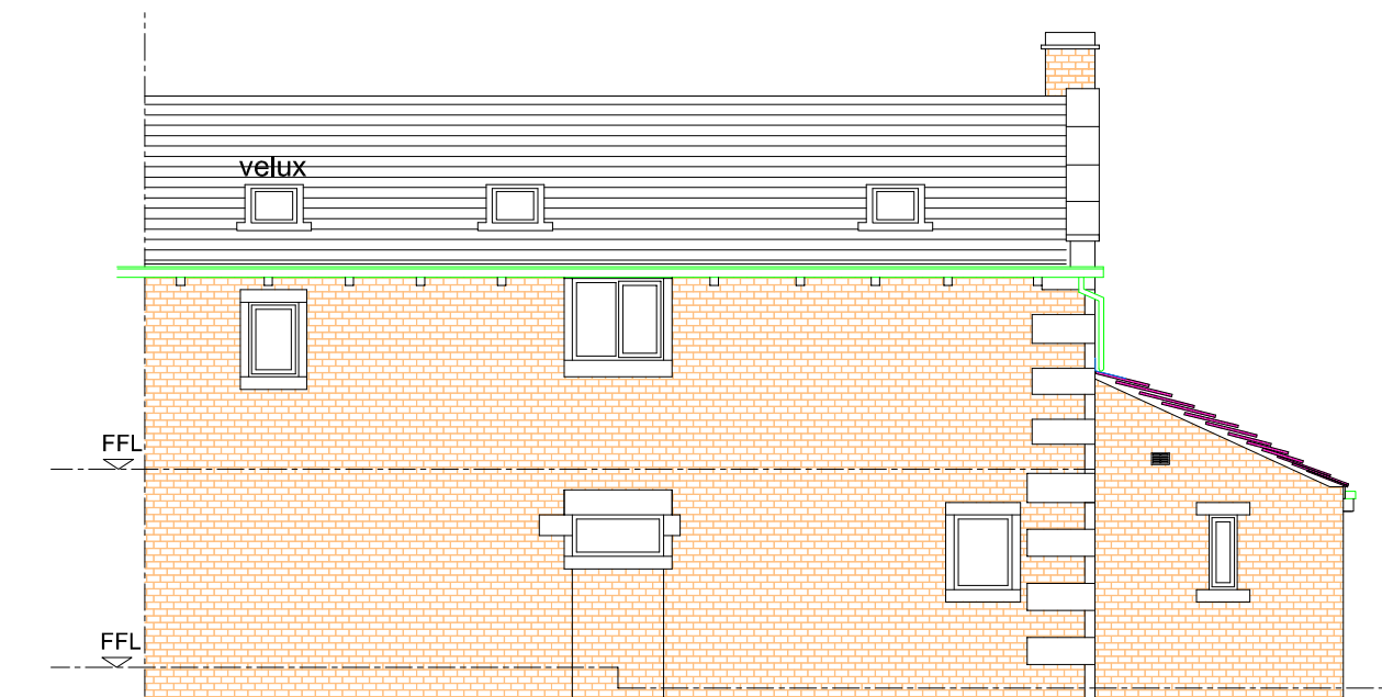
REAR ELEVATION AS PROPOSED (EAST) - 1:100
