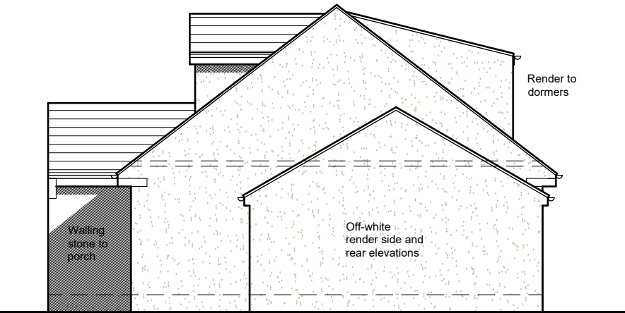
West Elevation
