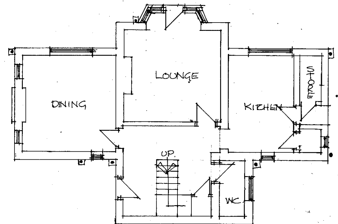
FRONT SIDE & REAR EXTENSIONS TO 12 CAWLEY LANE HECKMONDWIKE EX PLANS CLH/01
