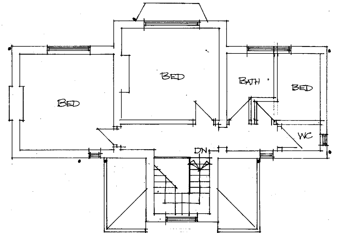
FIRST 1:100
