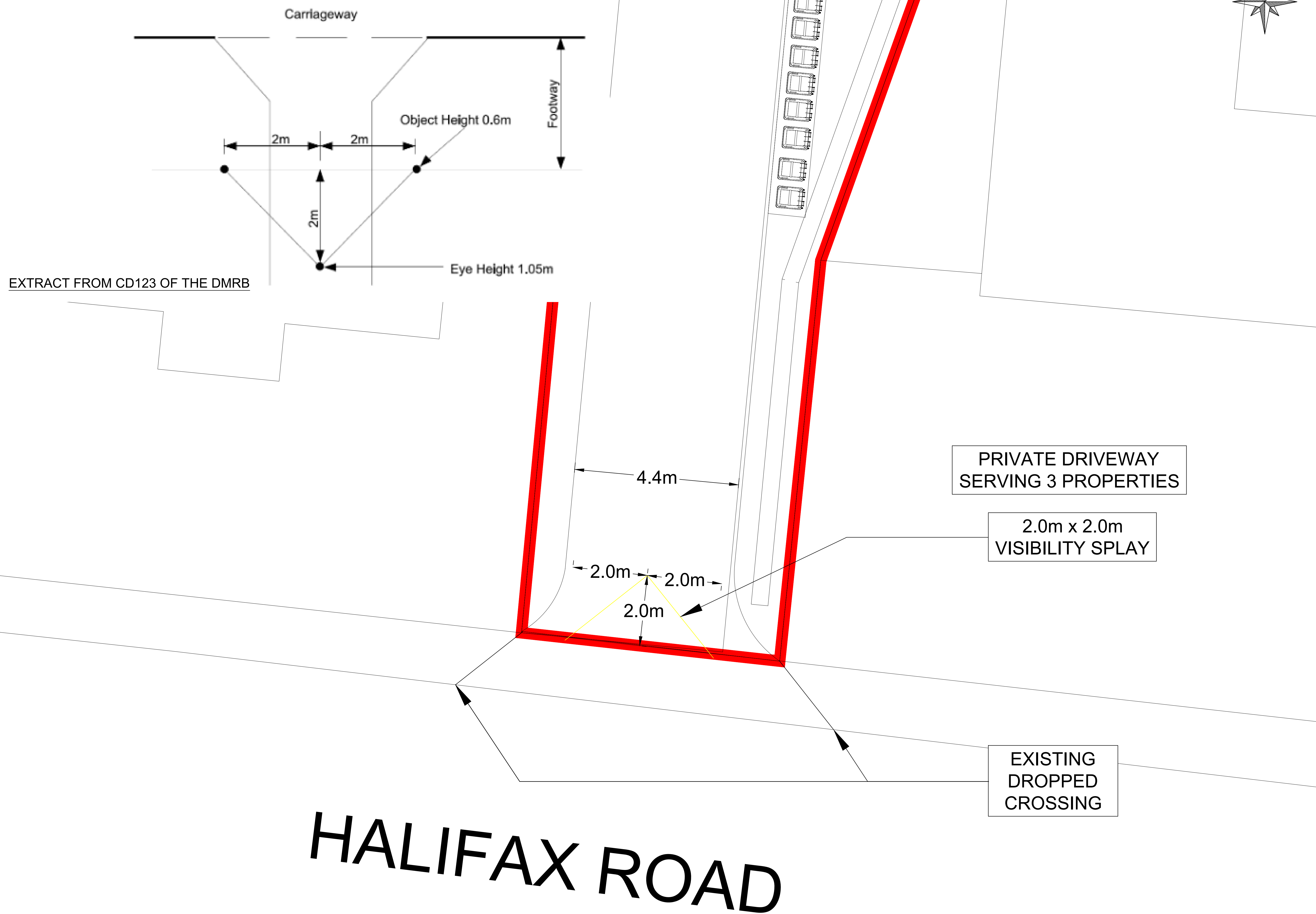
Figure 3.3 Visibility at the back of footway crossing
