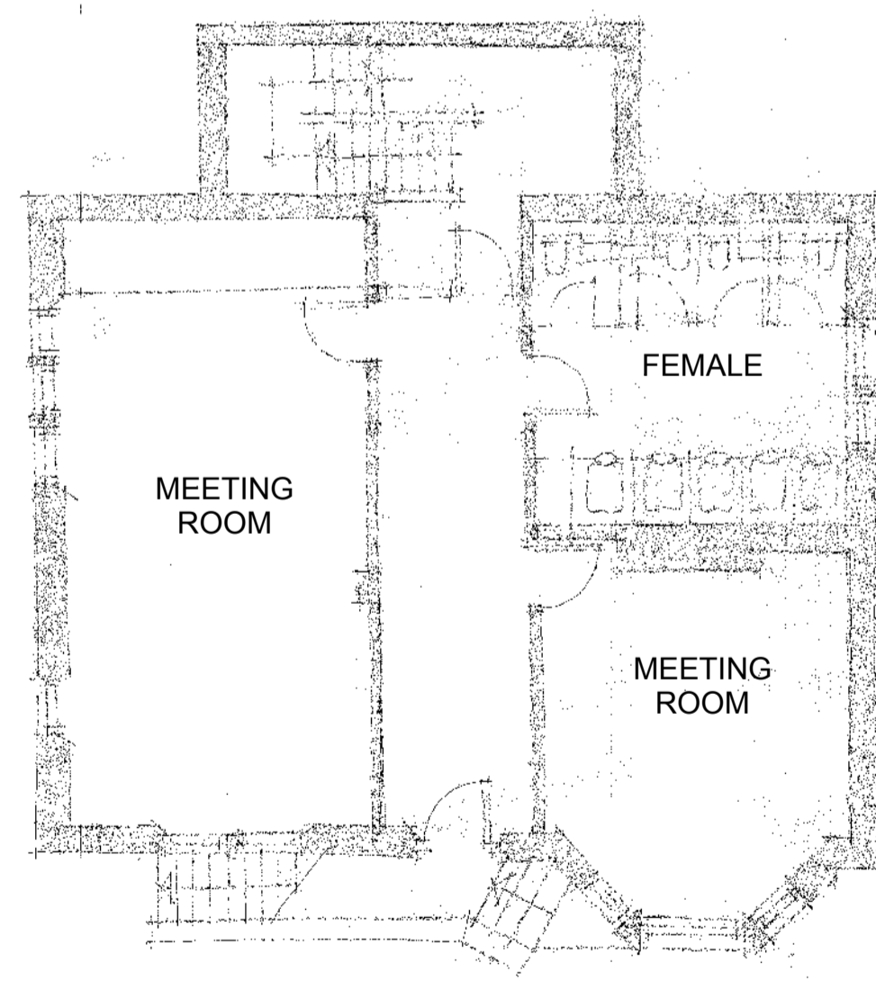
GROUND FLOOR PLAN - 1:100 PROPOSED
