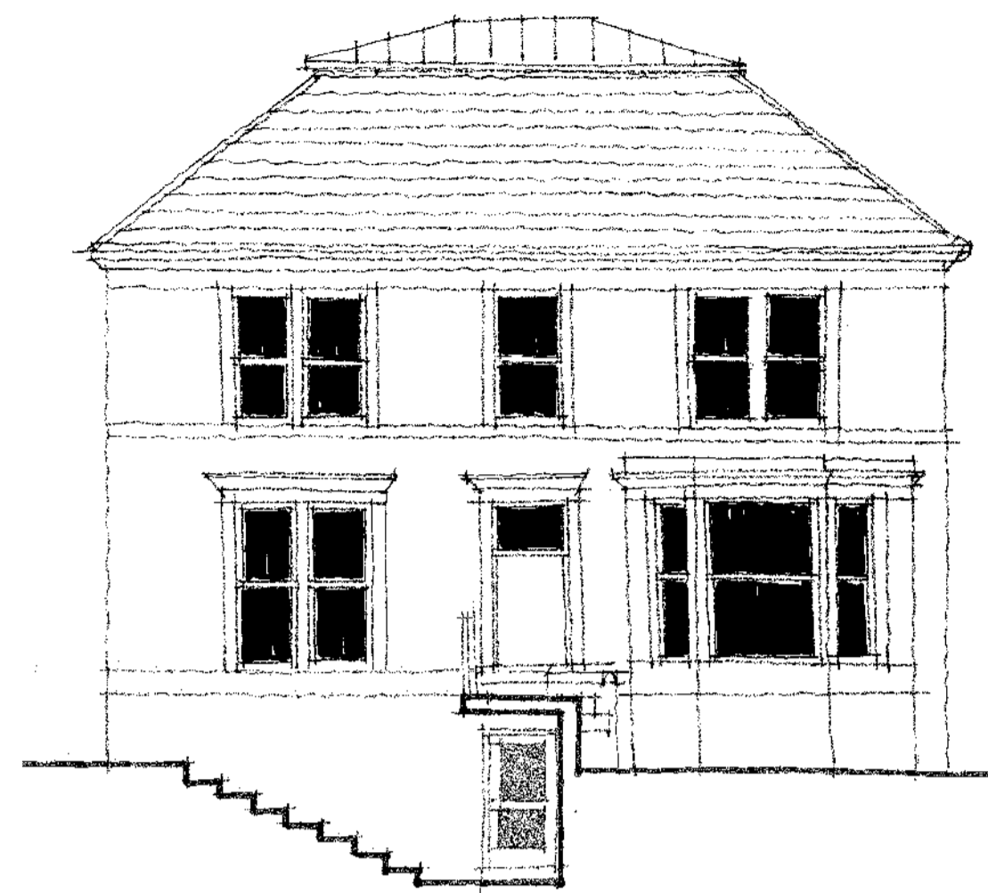
NORTH EAST ELEVATION - 1:100 PROPOSED
