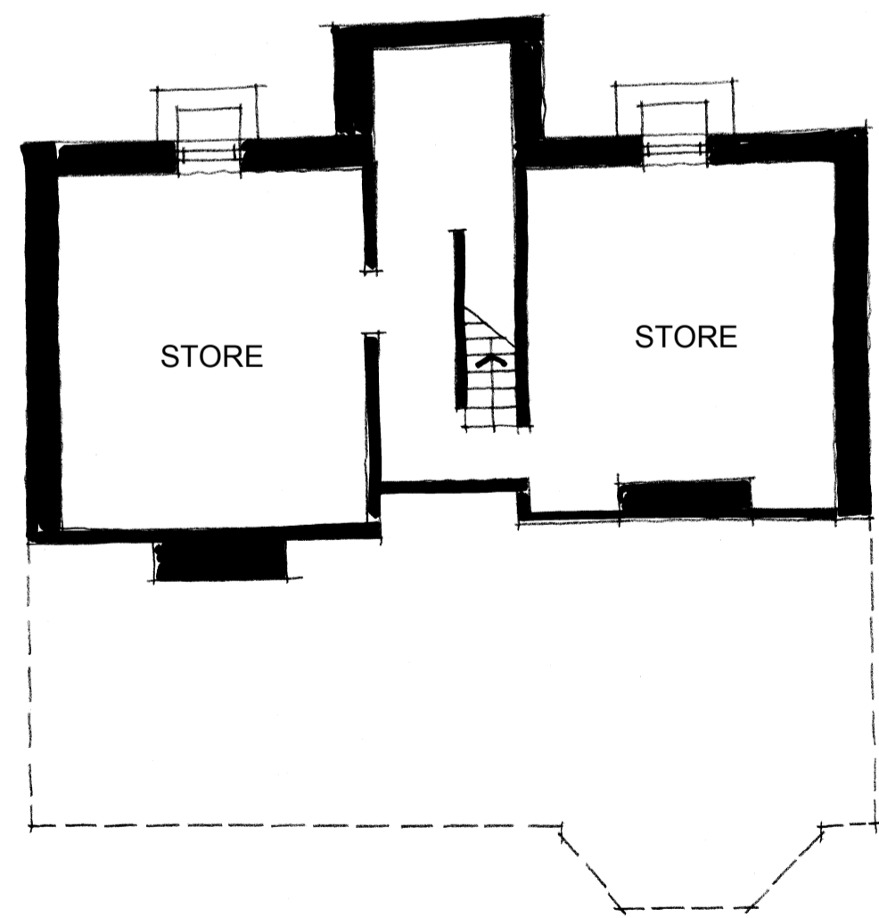
BASEMENT FLOOR PLAN - 1:100 EXISTING
