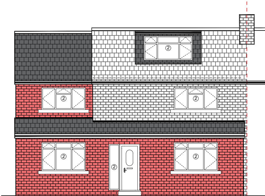
PROPOSED FRONT ELEVATION (SOUTH EAST)
