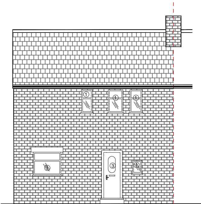
EXISTING FRONT ELEVATION (SOUTH EAST)
