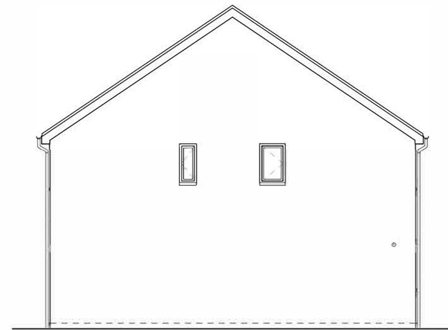
Side Elevation (Semi/End Terrace) 1 : 100
