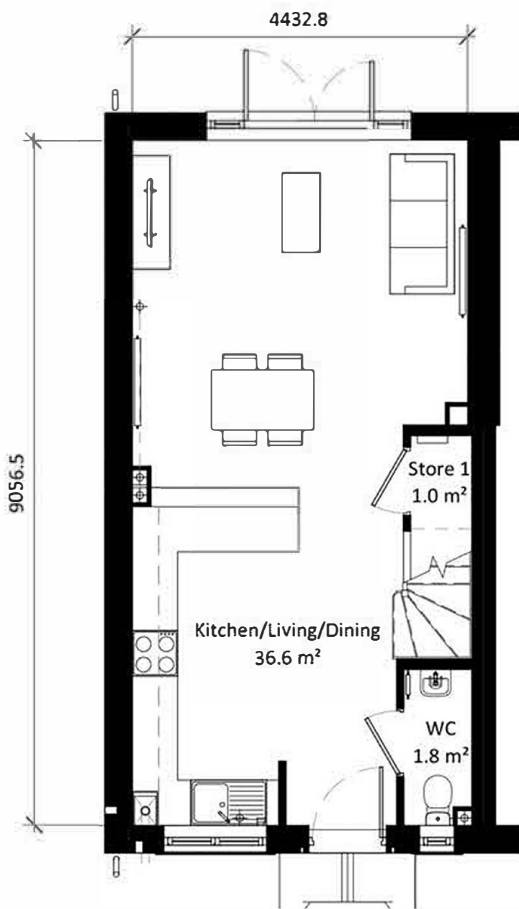
Ground Floor 1 : 100
