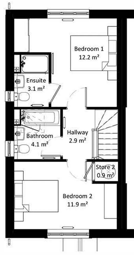
First Floor 1 : 100
