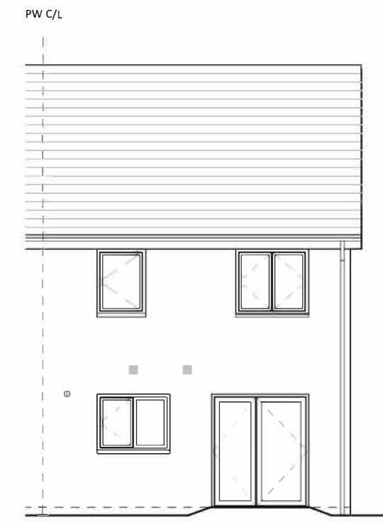
Rear Elevation 1 : 100
