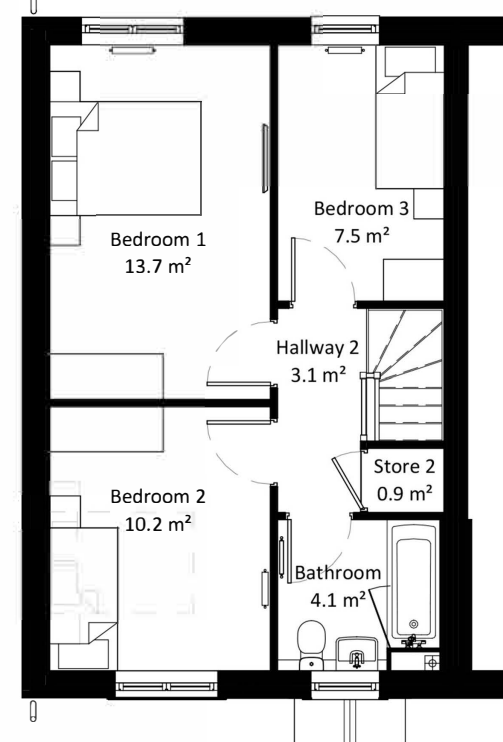
First Floor 1 : 100
