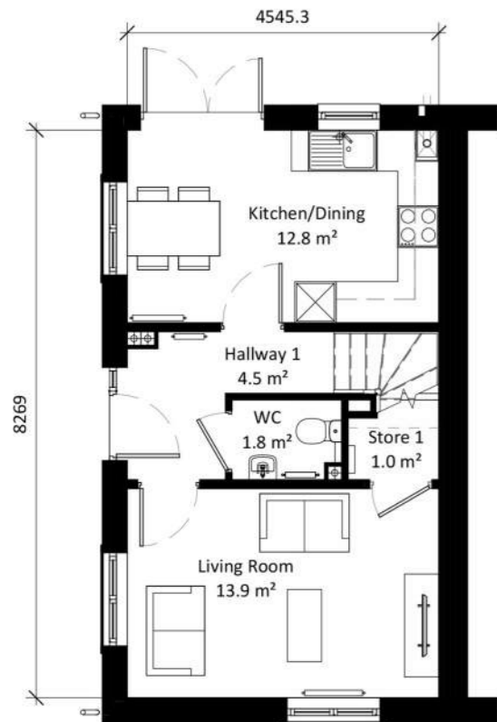
Ground Floor 1 : 100
