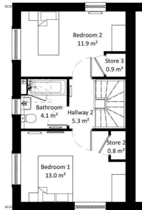
First Floor 1 : 100
