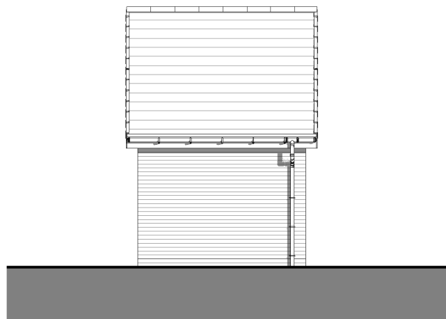
REAR ELEVATION
