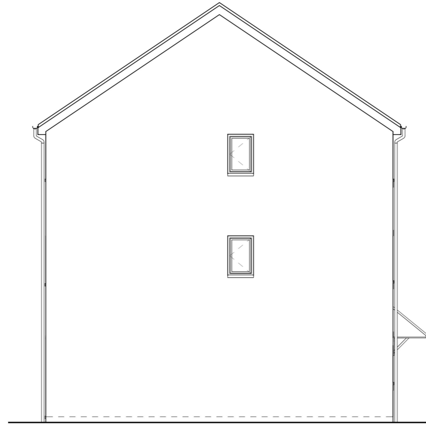
Side Elevation (Semi/End Terrace)
