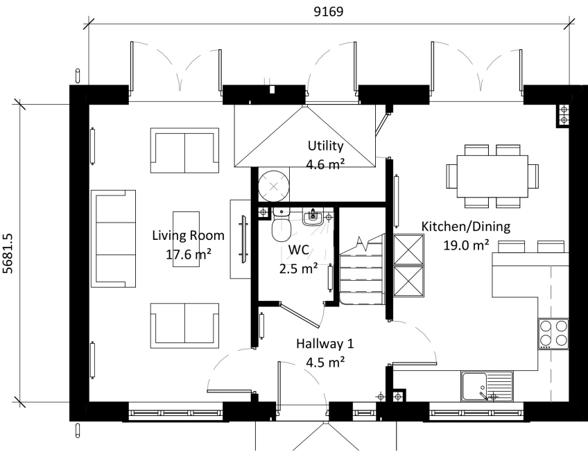
Ground Floor 1 : 100
