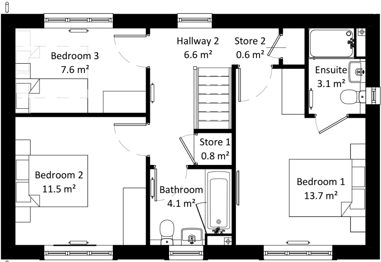
First Floor 1 : 100
