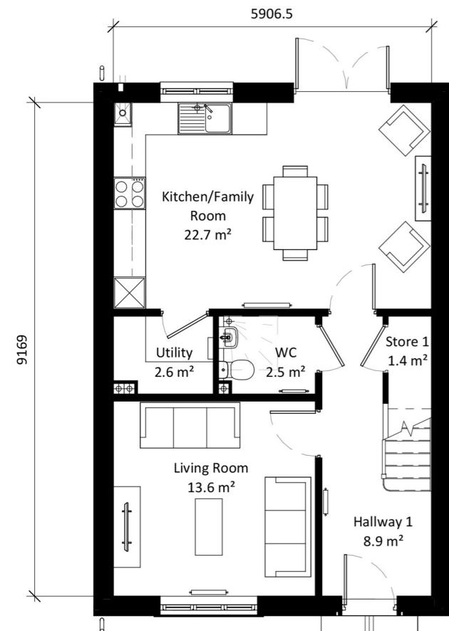
Ground Floor 1 : 100
