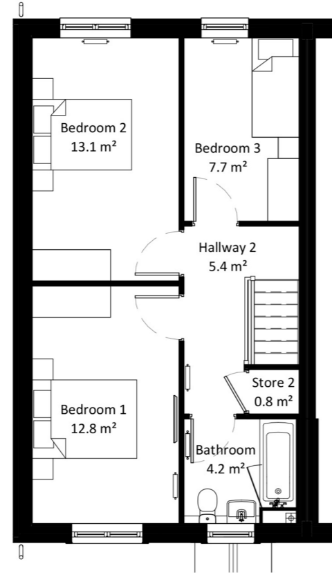
First Floor 1 : 100
