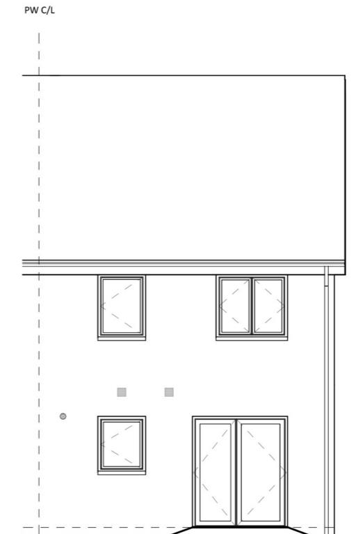
Rear Elevation 1 : 100
