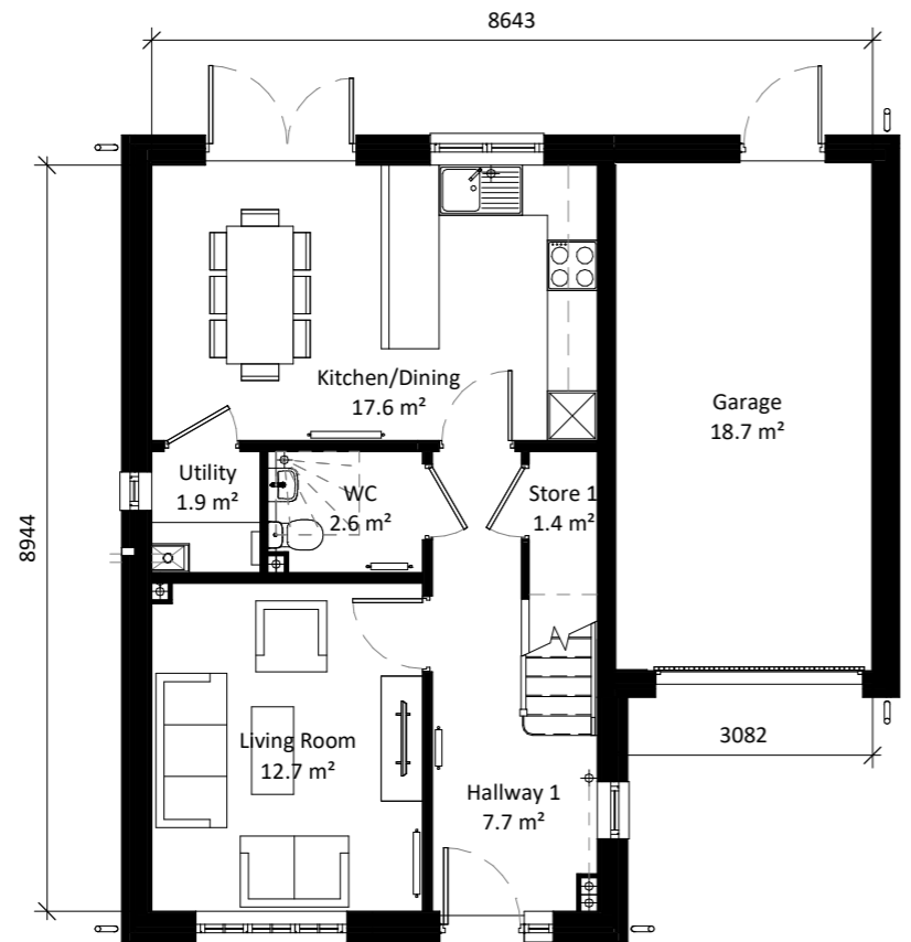
Ground Floor 1 : 100
