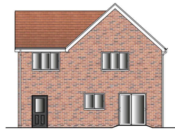
Rear Elevation 1 : 150
