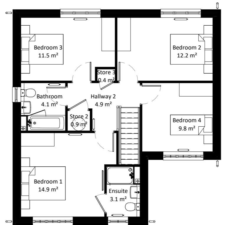
First Floor 1 : 100
