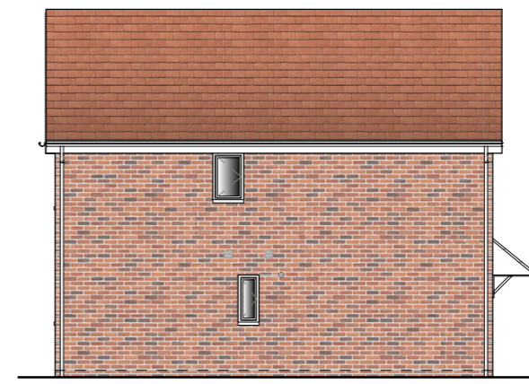
Side Elevation 1 : 150
