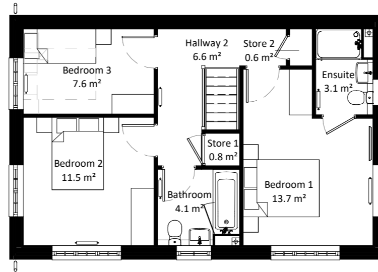
First Floor 1 : 100
