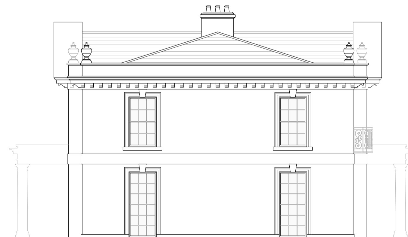
WEST ELEVATION
