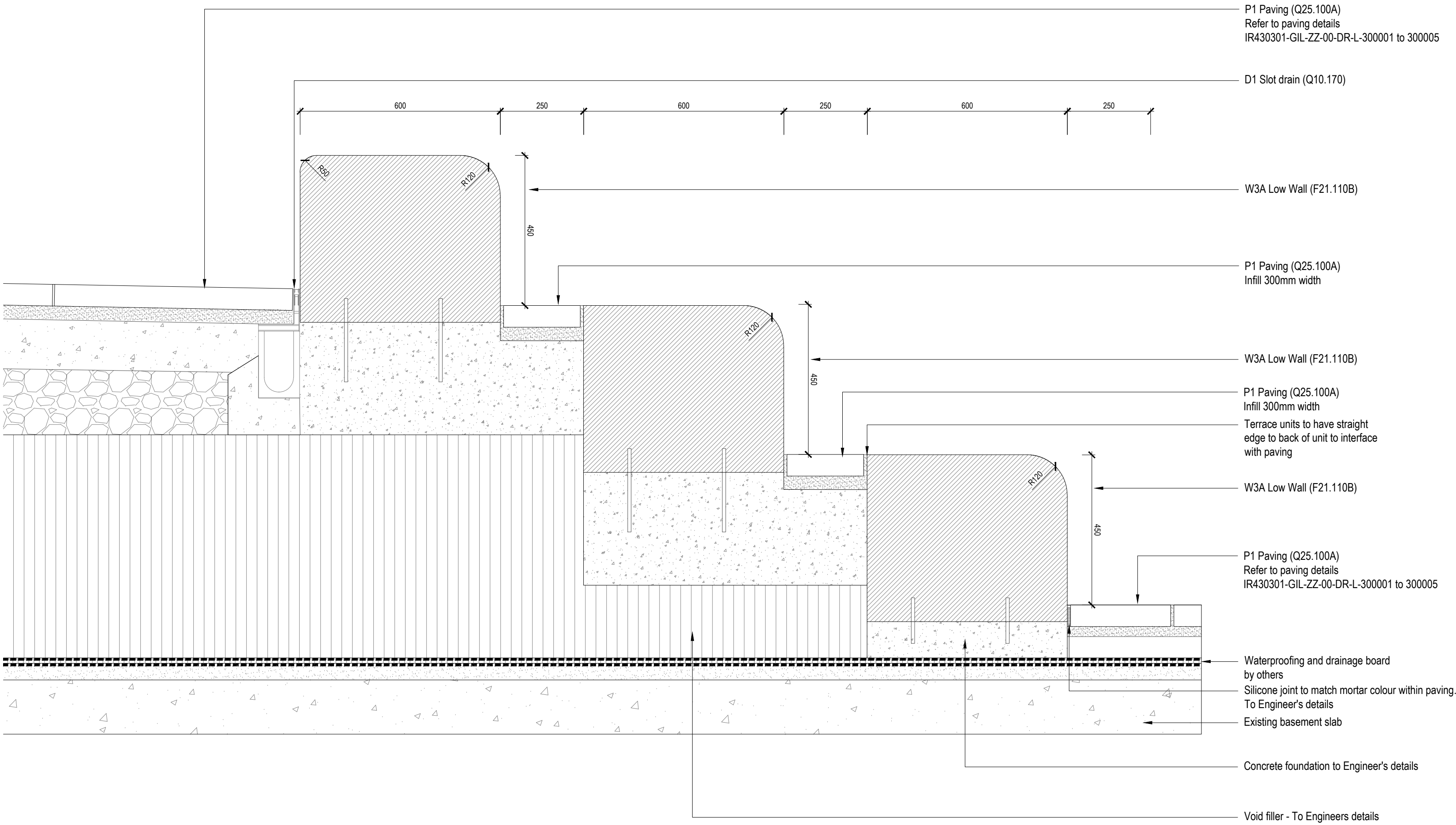
01 310012 W3A WALL UNIT STACKED Scale 1: 10 @A1
