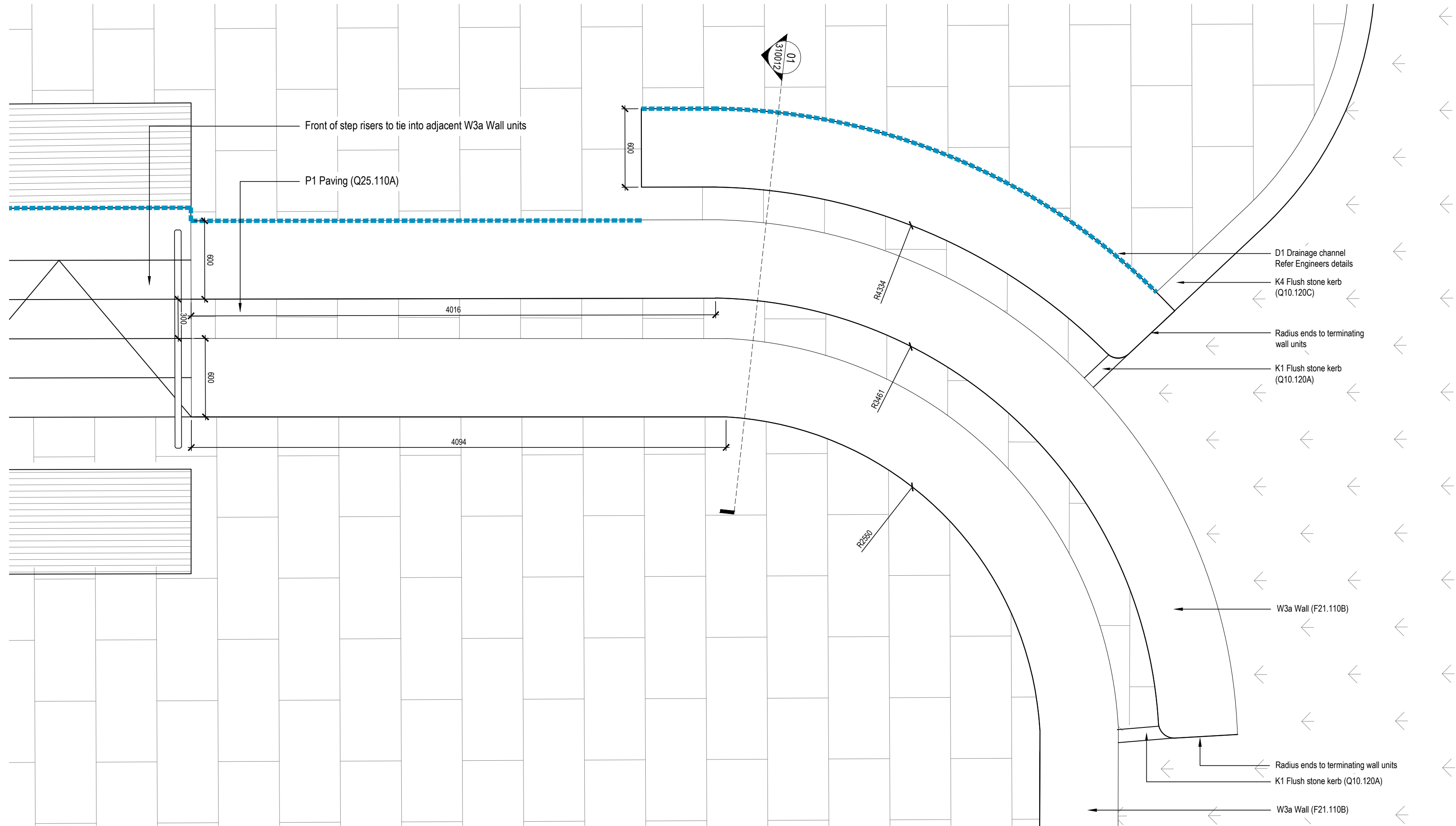
02 310012 W3A WALL UNIT STACKED - PLAN VIEW Scale 1: 25 @A1
