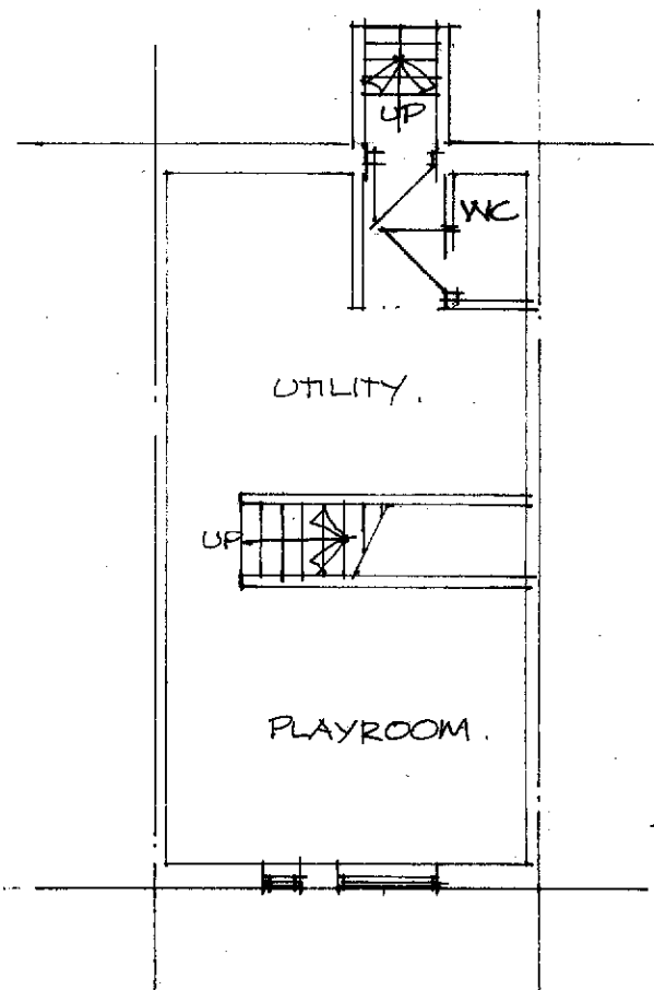
BASEMENT 1:100
