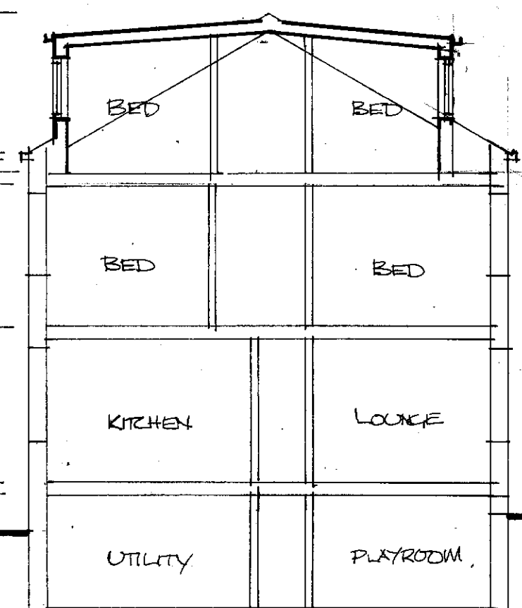
SECTION 1:100
