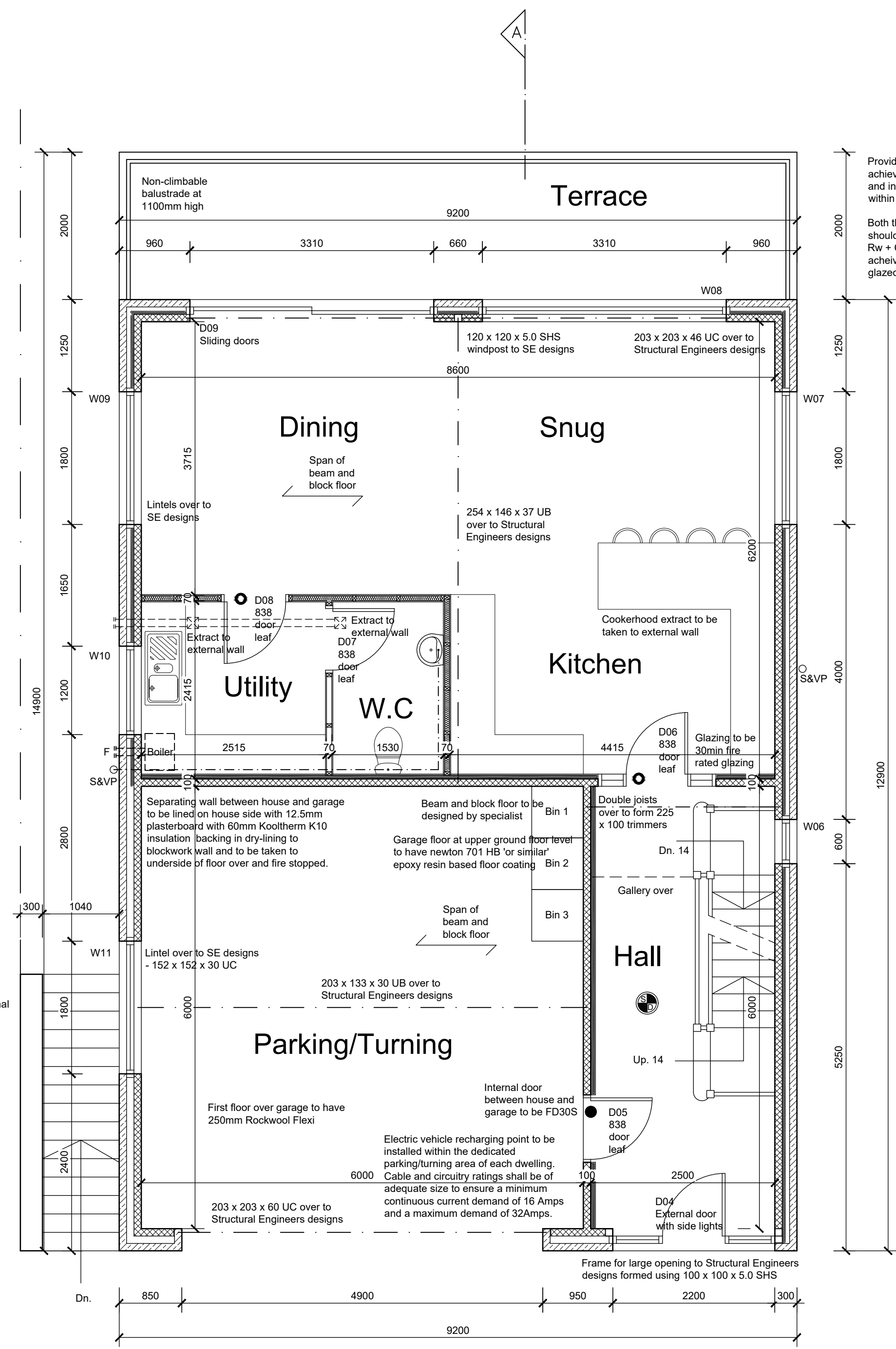
Upper Ground Floor Plan
