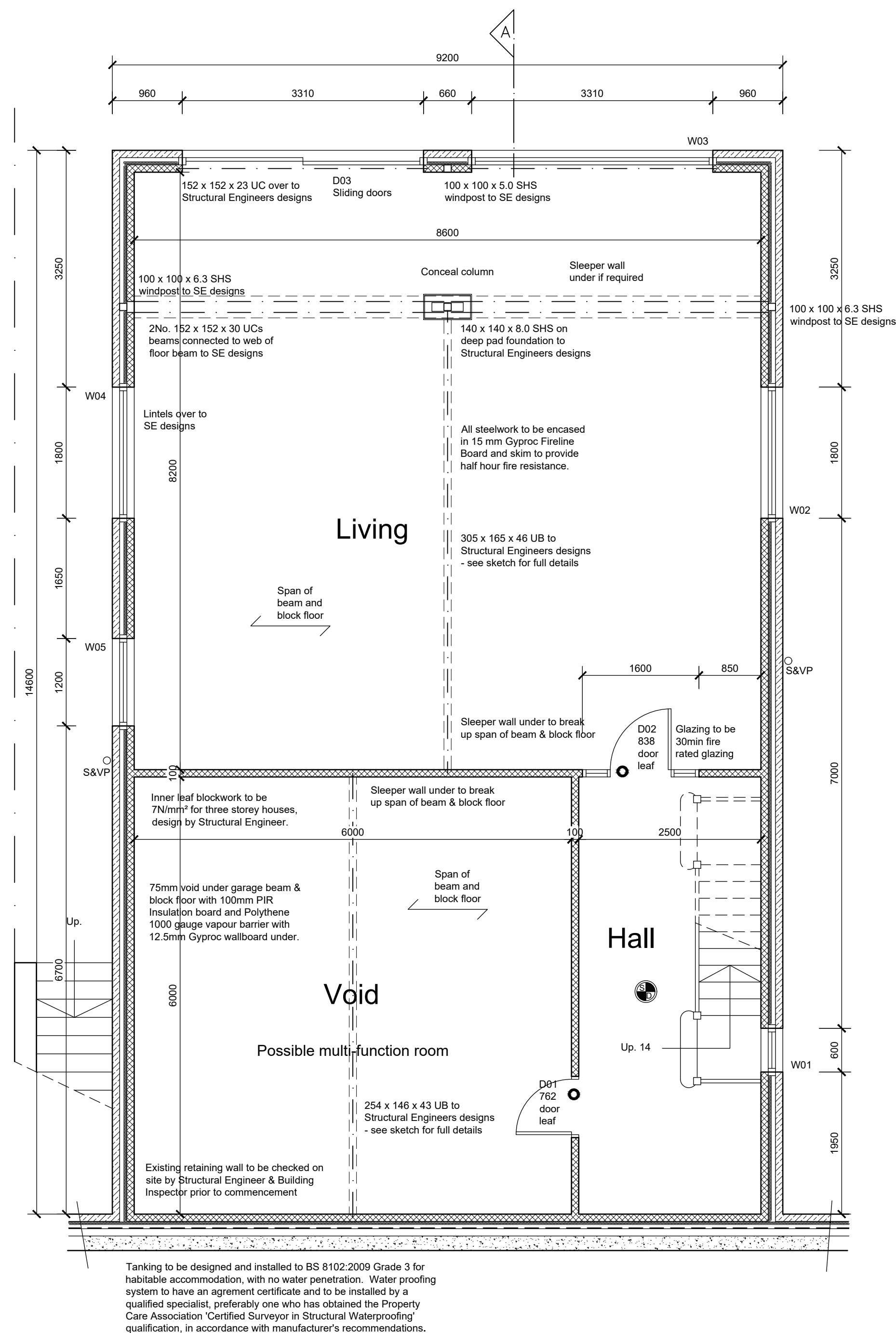
Lower Ground Floor Plan
