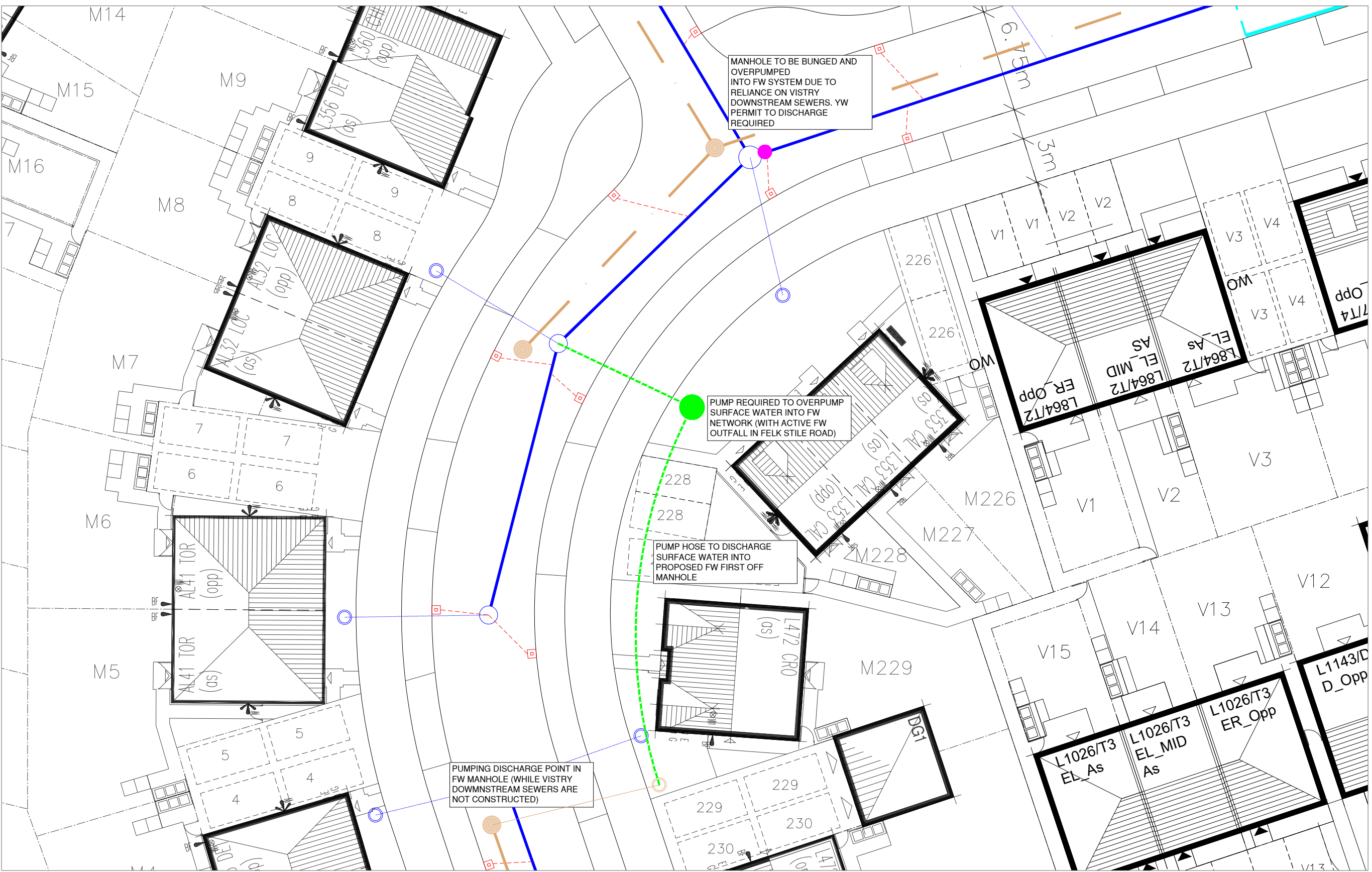
TEMPORARY SURFACE WATER OVERPUMPING (WHEN DOWNSTREAM SEWERS ARENT CONSTRUCTED BY VISTRY HOMES)
