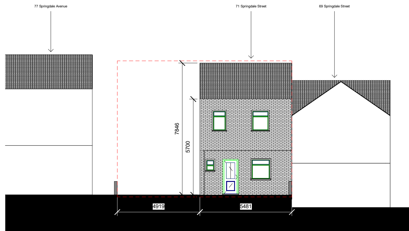
Existing Back Elevation East Facing Elevation
