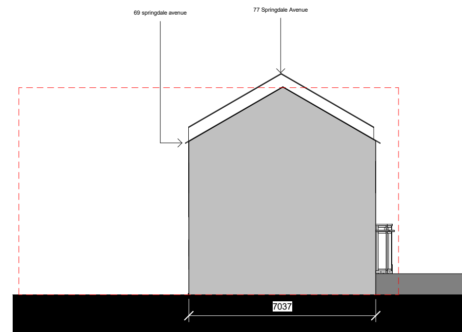
Existing Side Elevation North Facing Elevation
