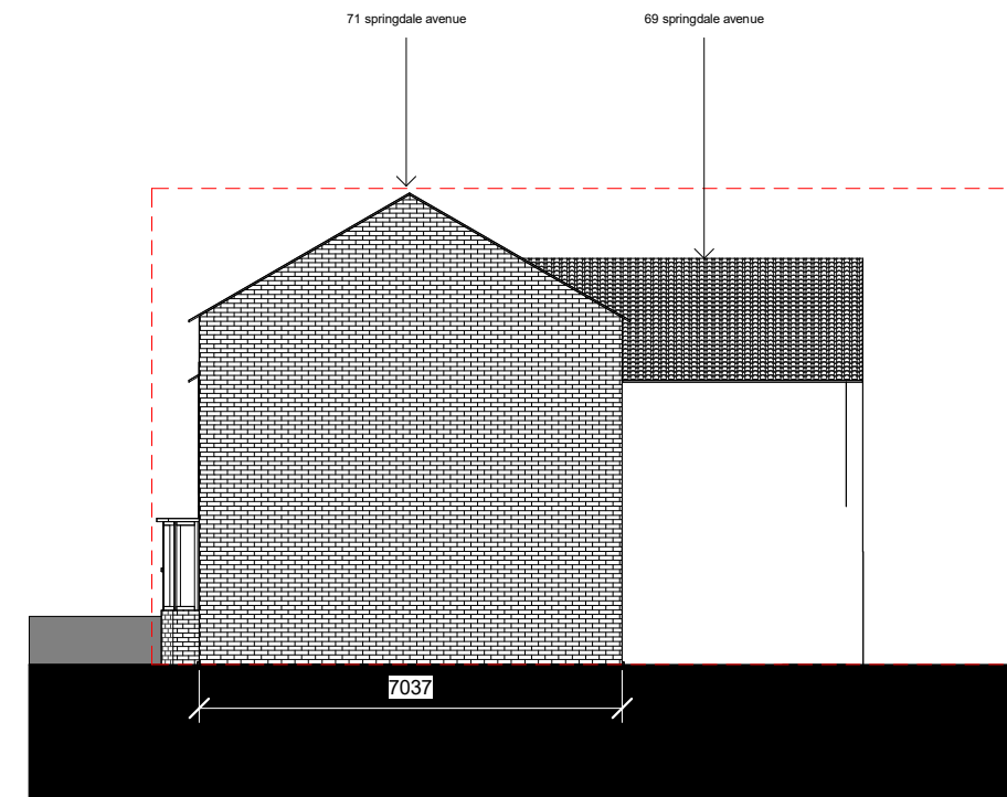
Existing Side Elevation South Facing Elevation
