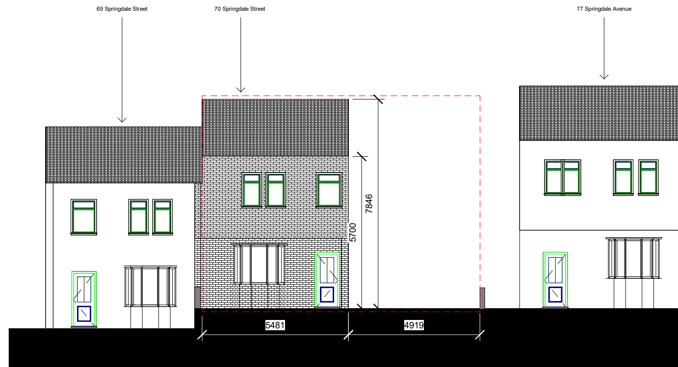
Existing Front Elevation West Facing Elevation
