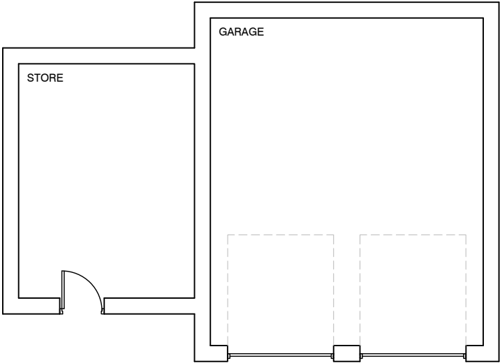
Proposed Floor Plans Of Building Cluster B 1:100
