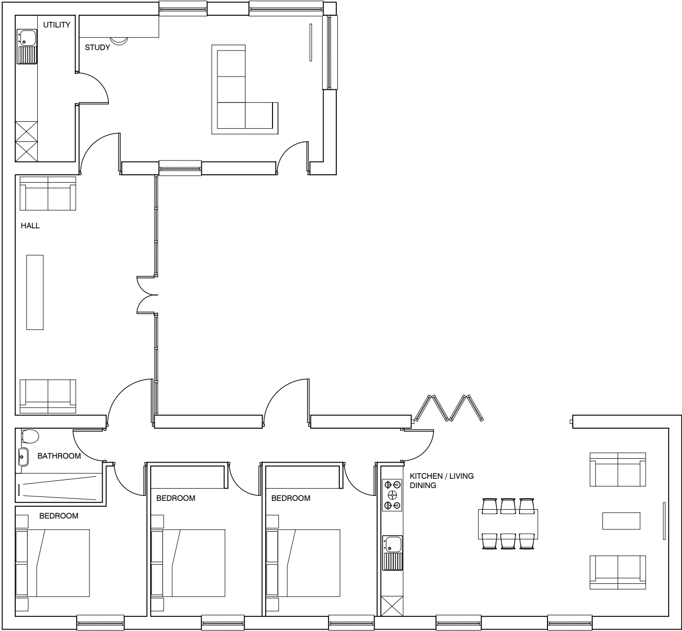
Proposed Floor Plans Of Building Cluster A 1:100
