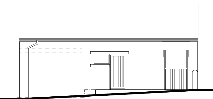
West Elevation - Existing
