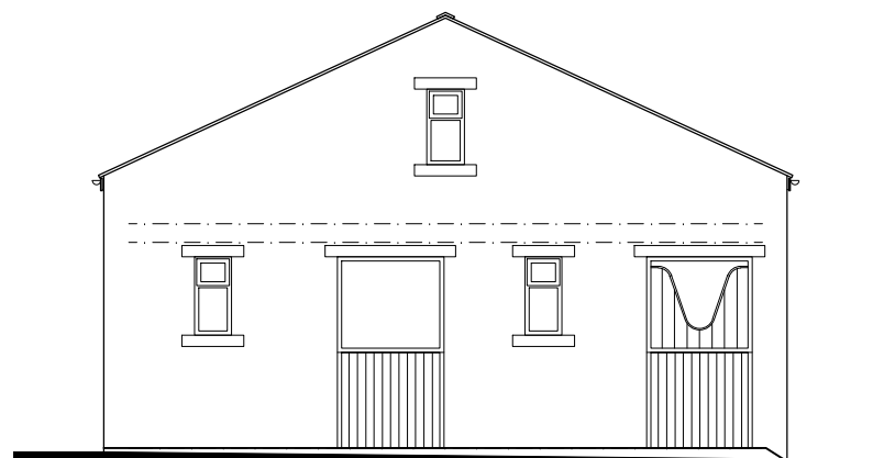
North Elevation - Existing
