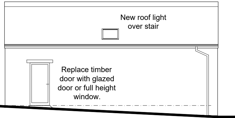
East Elevation
