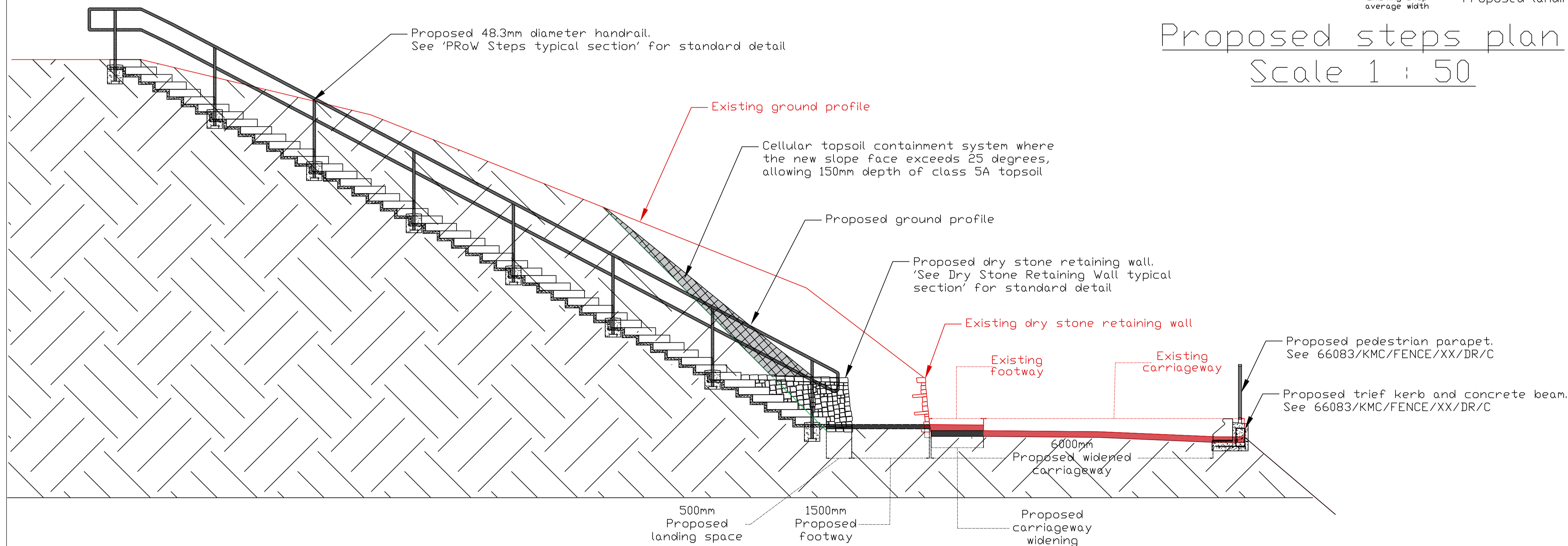
Proposed steps section Scale 1 : 50
