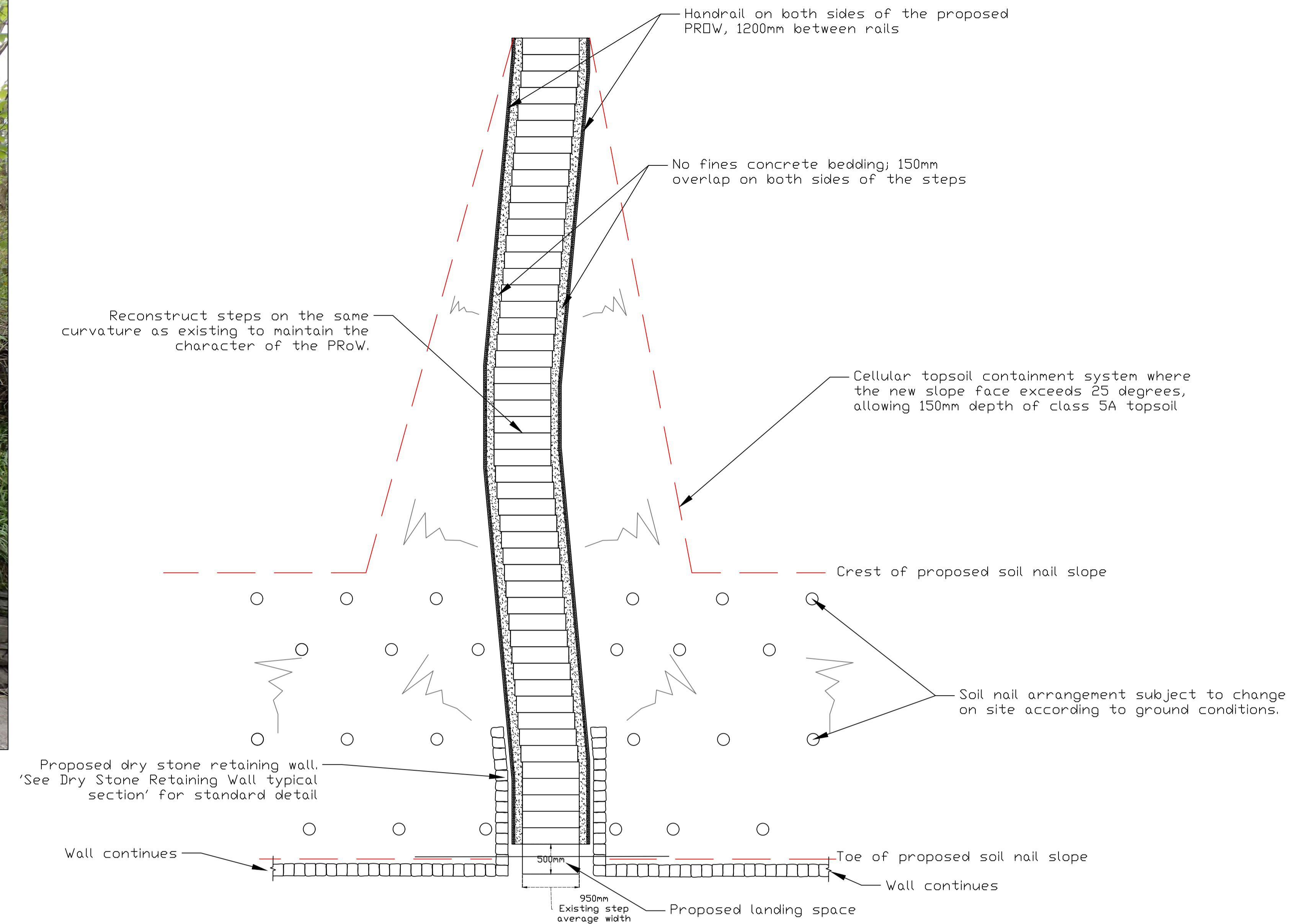
Proposed steps plan Scale 1 : 50
