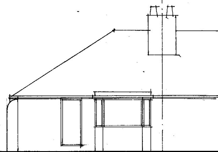
REAR 1:100
