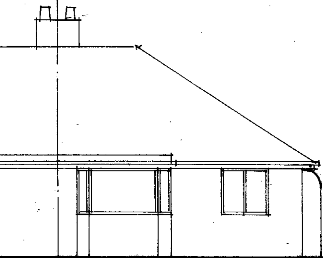
FRONT 1:100
