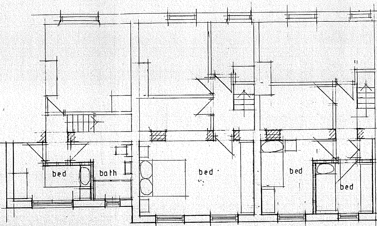
FIRST FLOOR
