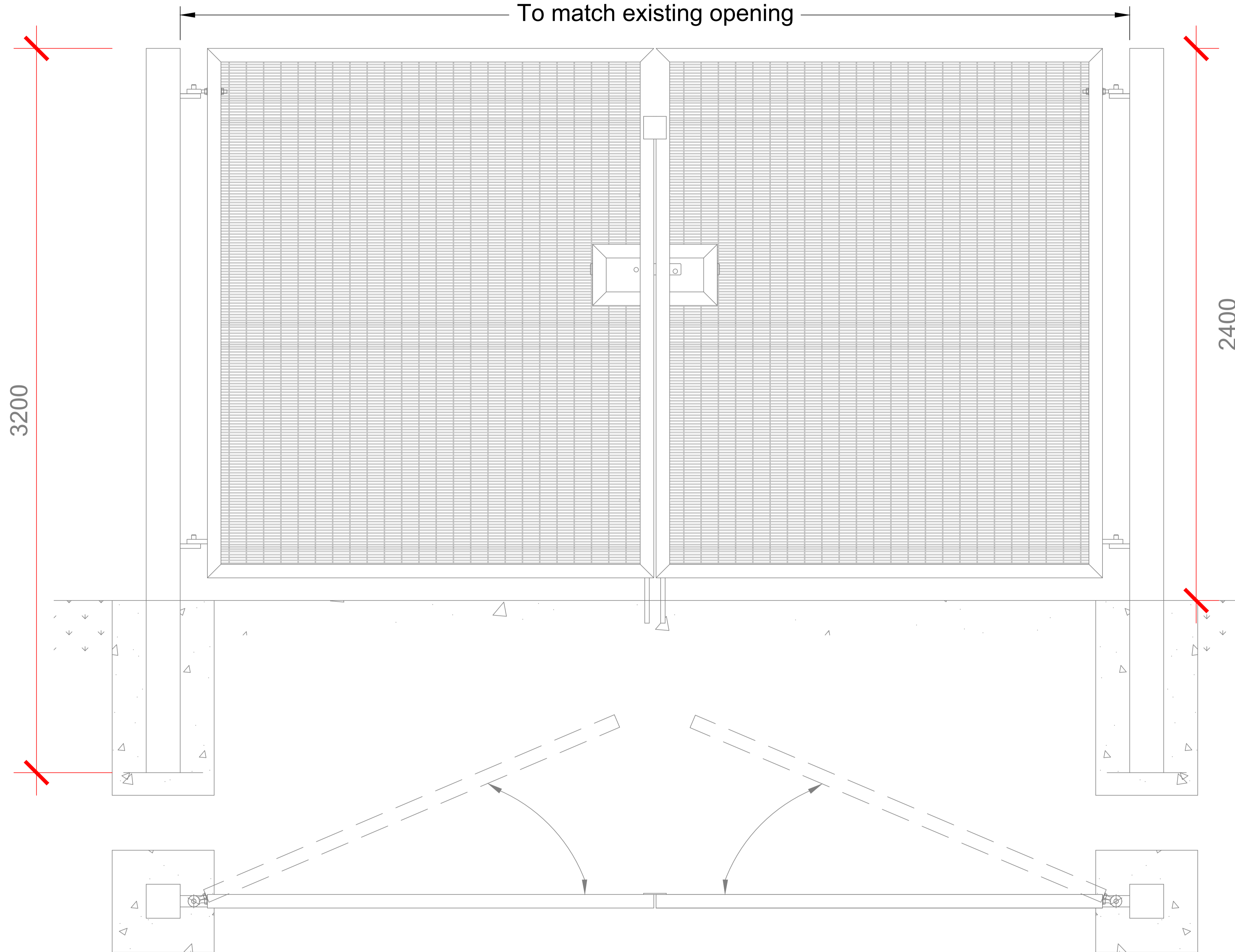
Gate Elevations Scale 1:10 @ A1
