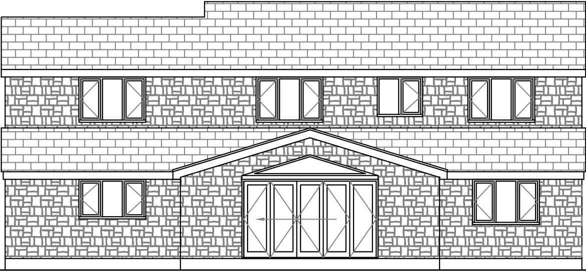
Rear Elevation
