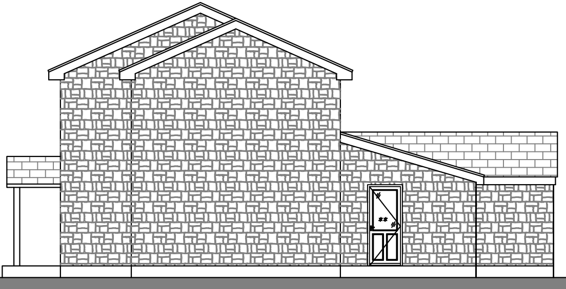
Side Elevation
