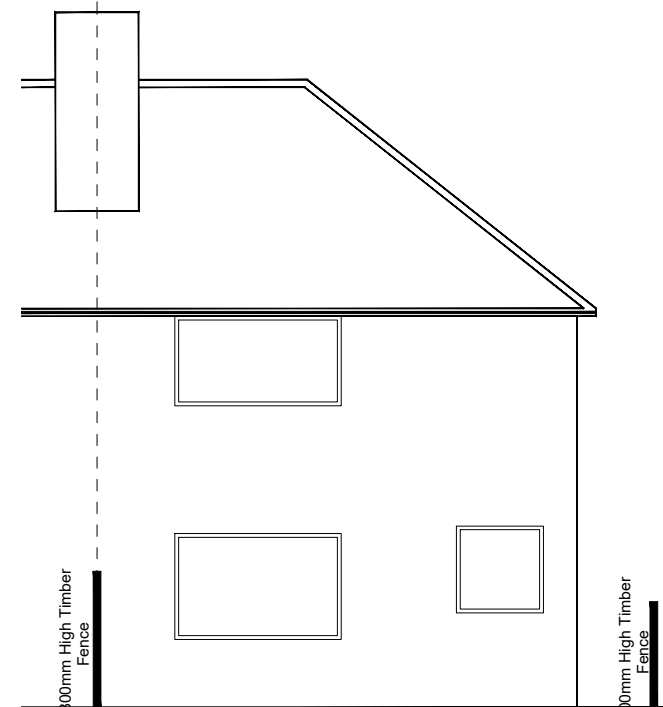
EXISTING REAR ELEVATION (SOUTH EAST ELEVATION)
