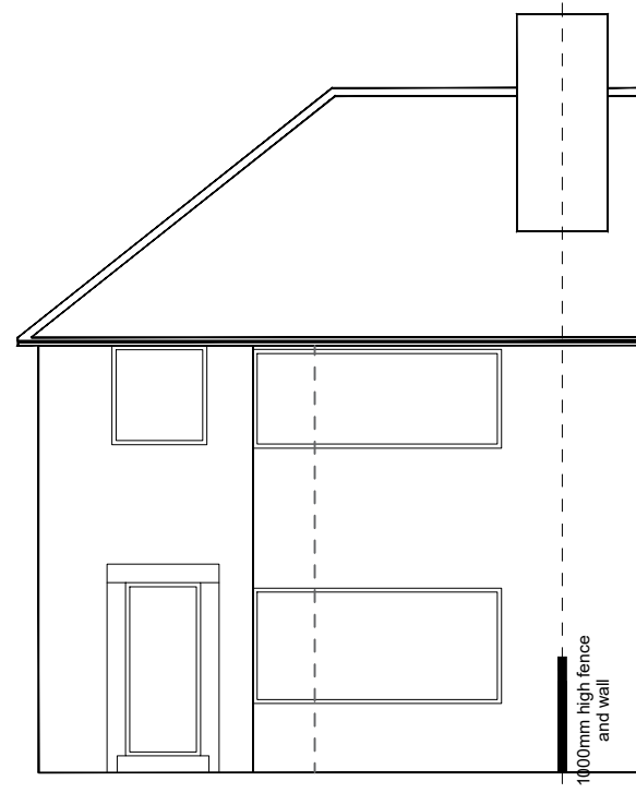
PROPOSED FRONT ELEVATION (NORTH WEST ELEVATION)
