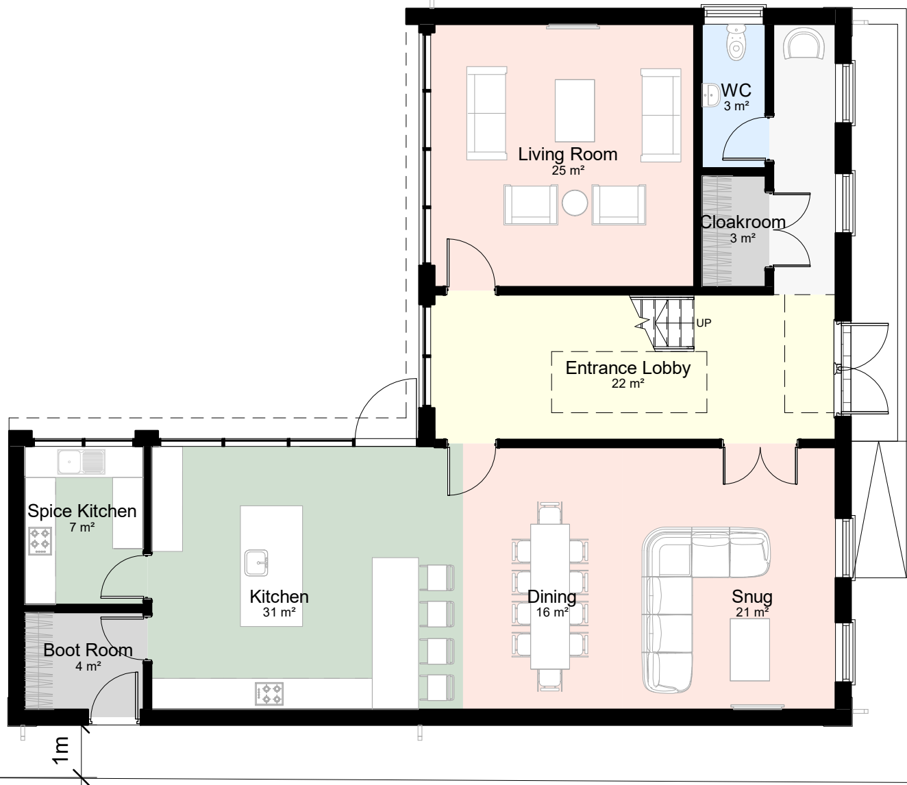
Proposed Ground Floor 1:100
