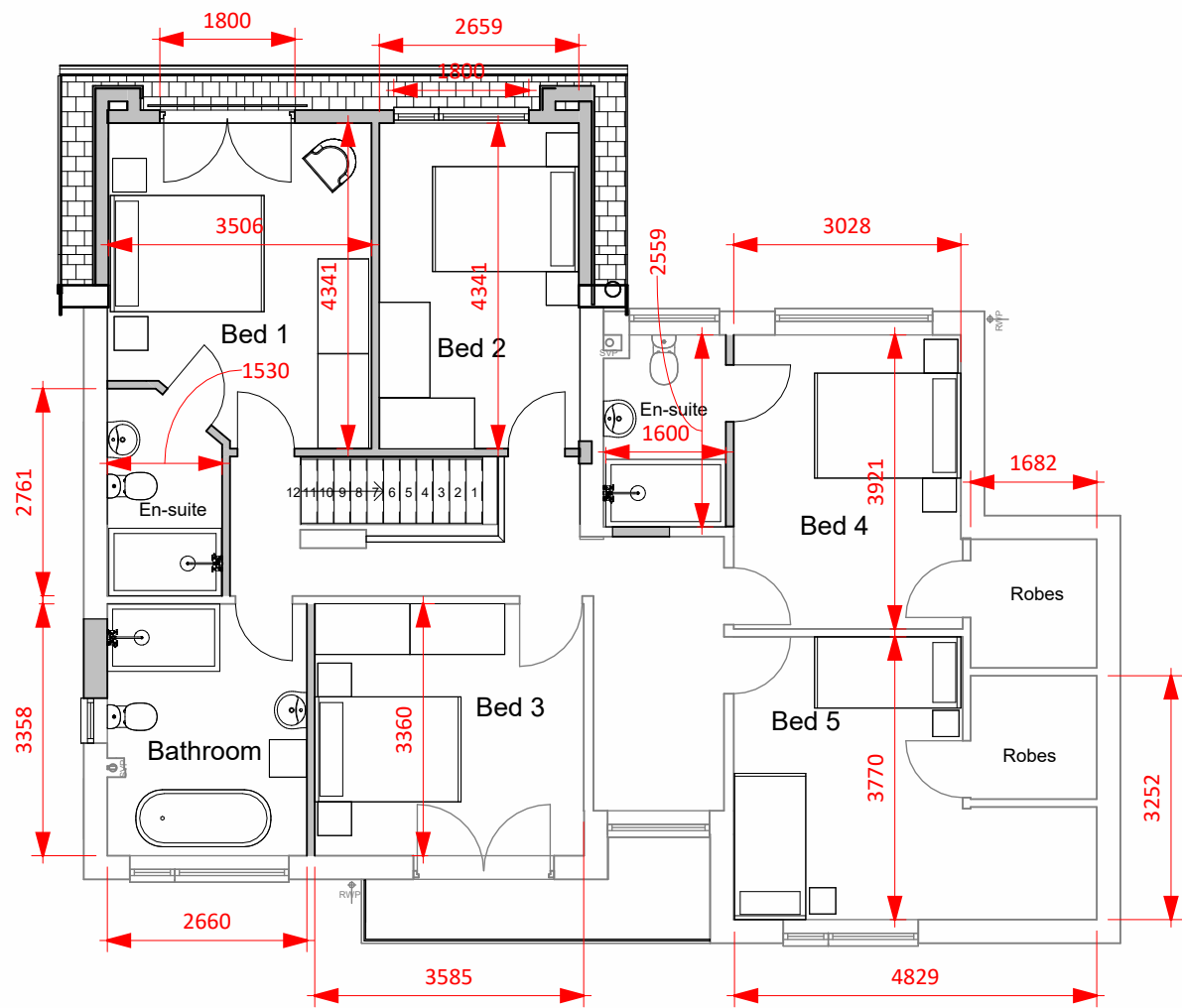
1 03b FF Proposed 1 : 100
