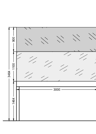
SIDE ELEVATION
