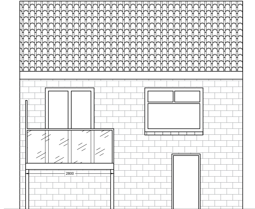
REAR ELEVATION
