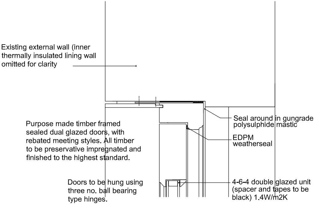
Head Detail 1:5 @ A2
