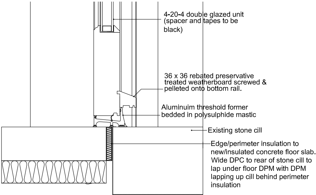
Sill Detail 1:5 @ A2
