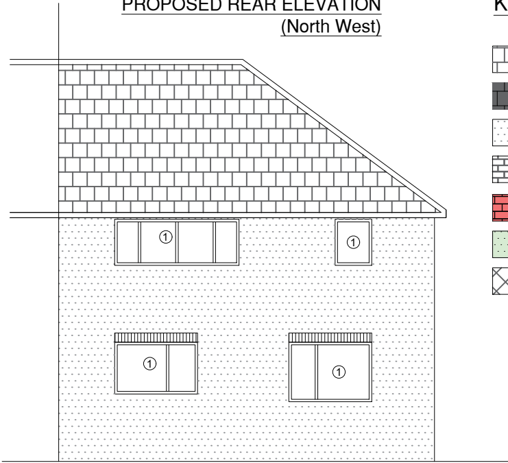
EXISTING REAR ELEVATION (North West)
