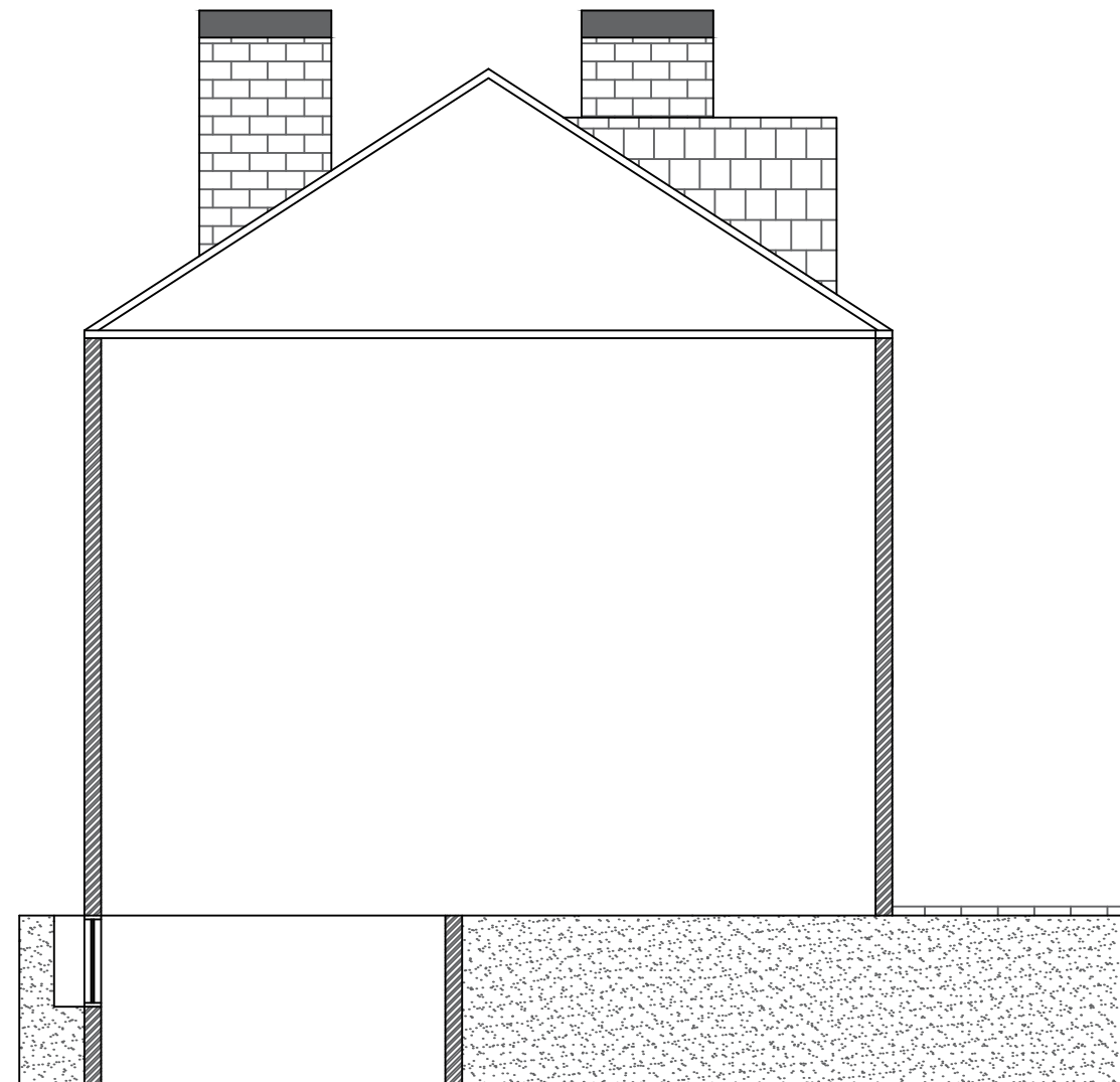
Existing East Elevation
