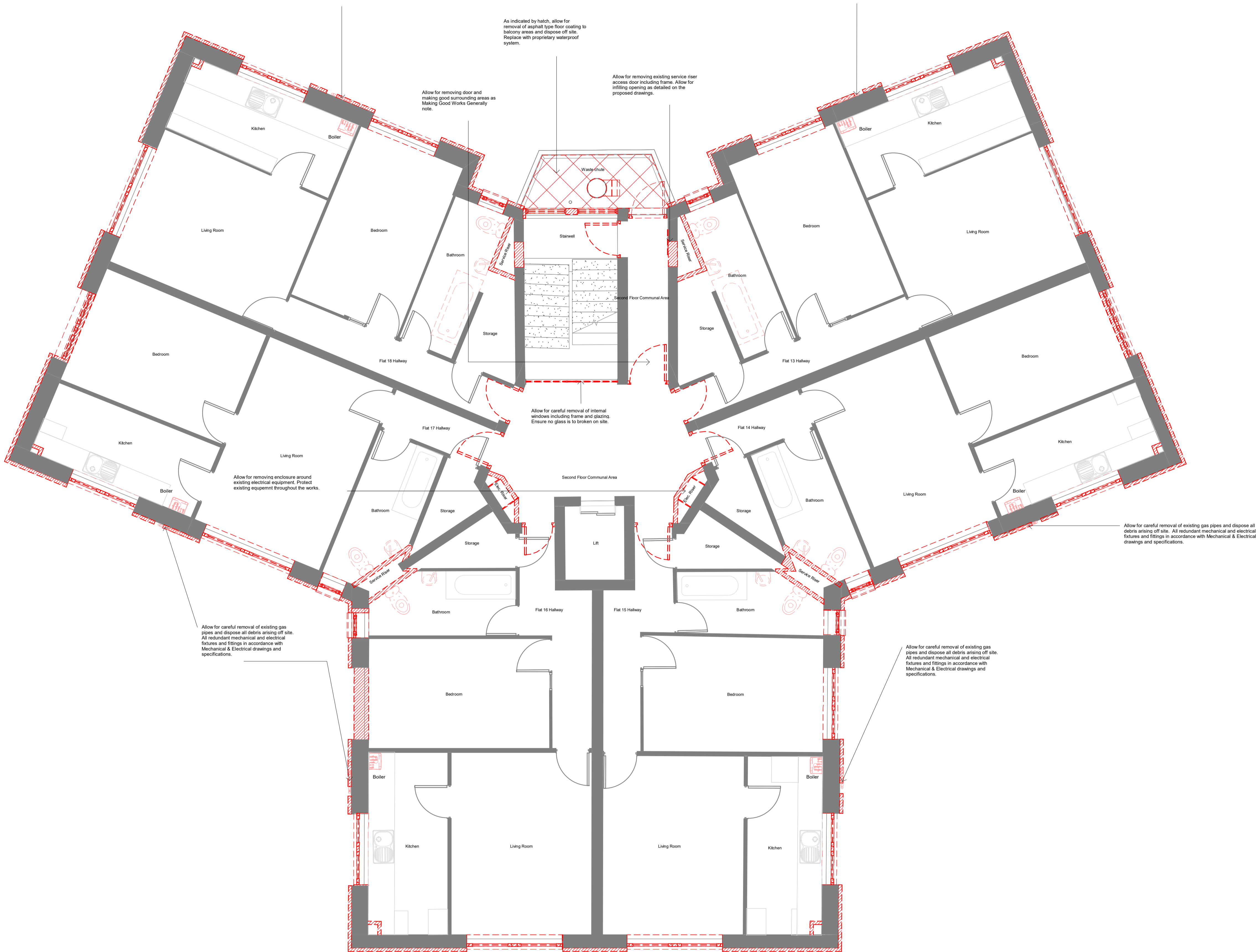
1 Existing - Second Floor Plan - Strip Out Works 1 : 50
