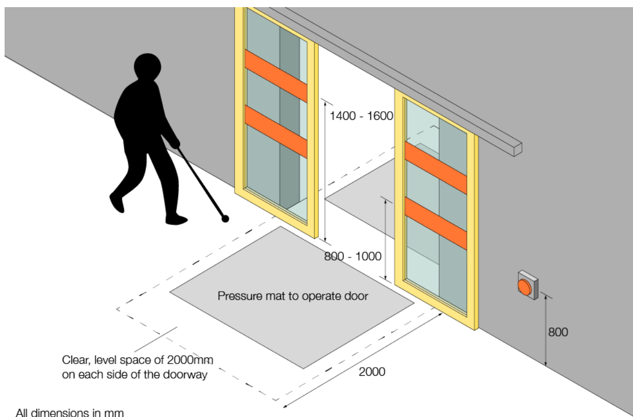
Figure 15: Automatic sliding doors
