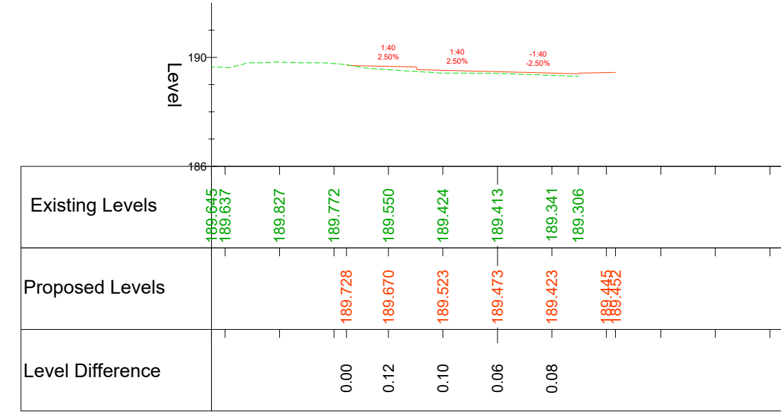
SHEPLEY ROAD - CROSS SECTIONS @ 20m-70m SCALE - 1:250
