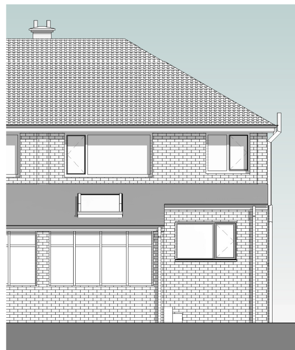
REAR ELEVATION AS EXISTING 1 : 100
