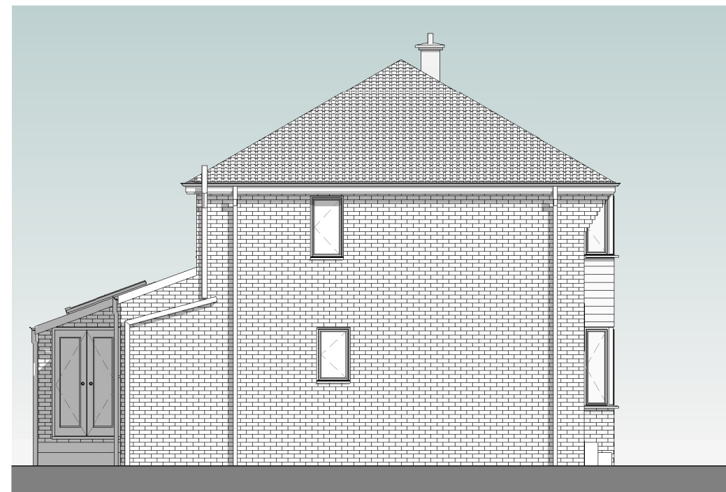
SIDE ELEVATION AS EXISTING 1 : 100
