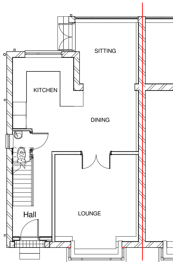
EXISTING GROUND FLOOR 1 : 100
