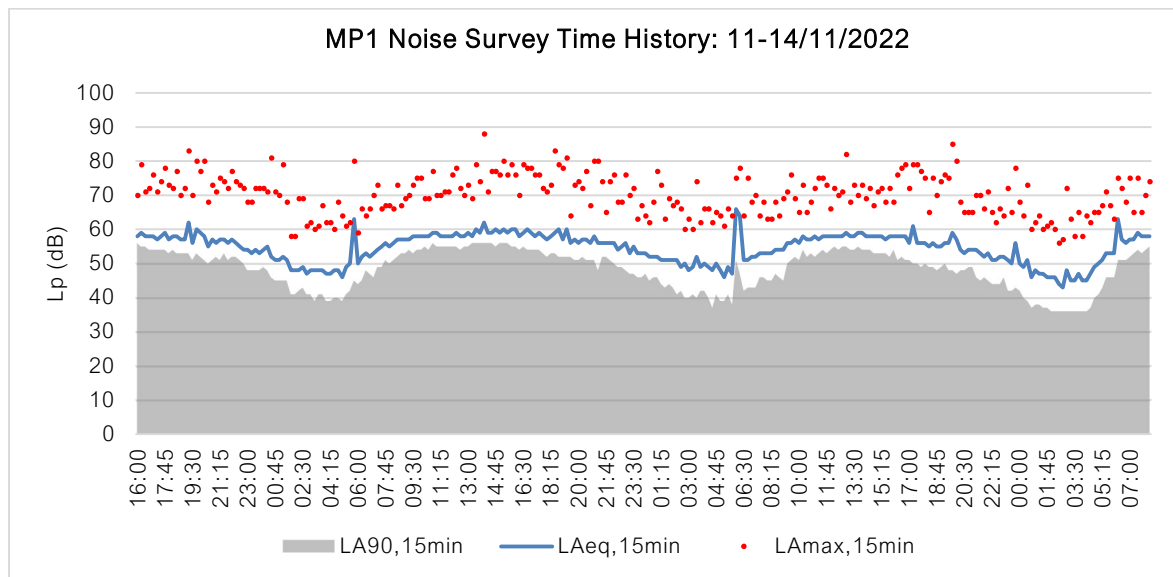
Figure 5 – MP1 Noise Survey Time History
