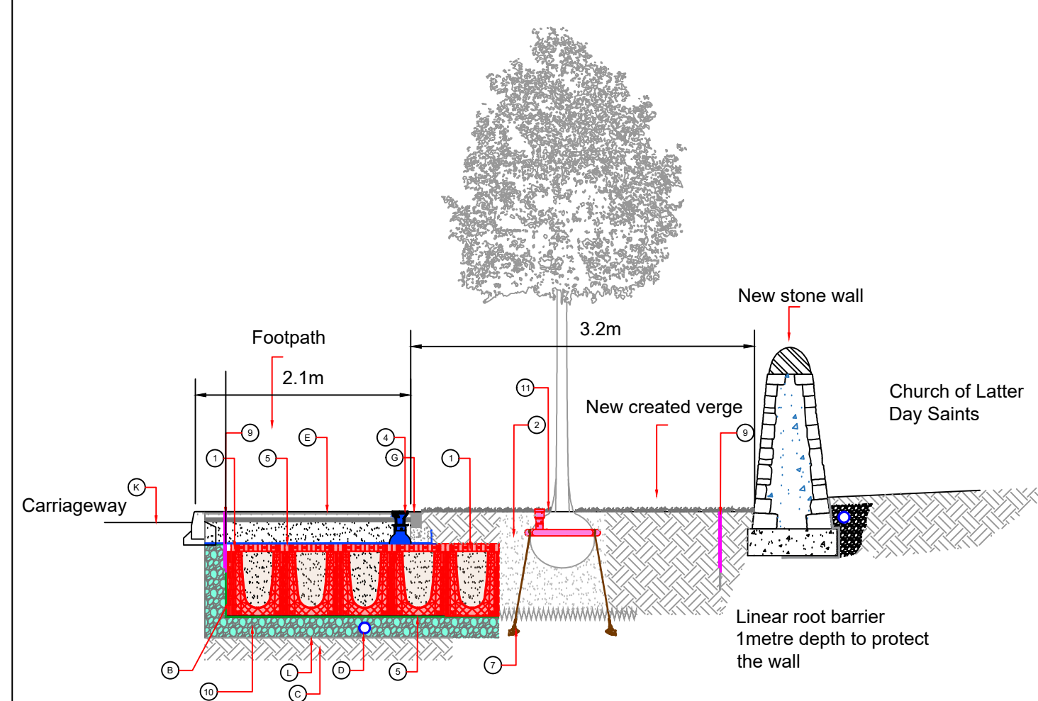
SECTION A-A For details refer to Landscape drawing: TF5-AREA D LSC-SD-4
