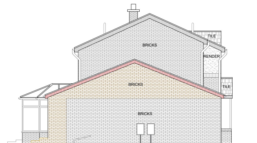
PROPOSED SIDE ELEVATION-2
