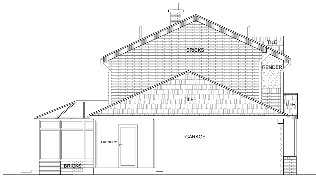
EXISTING SECTION
