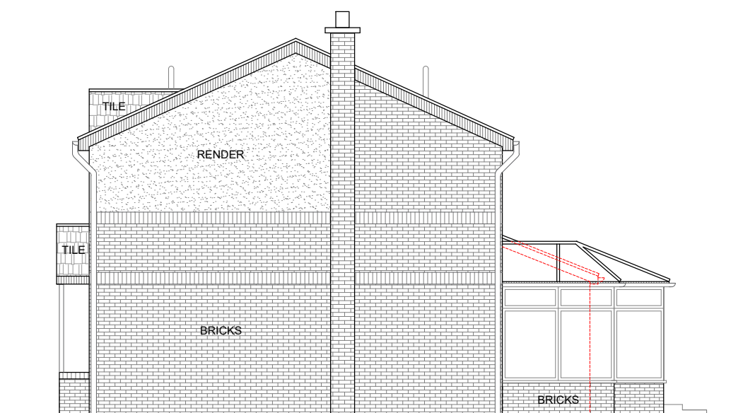
PROPOSED SIDE ELEVATION-1
