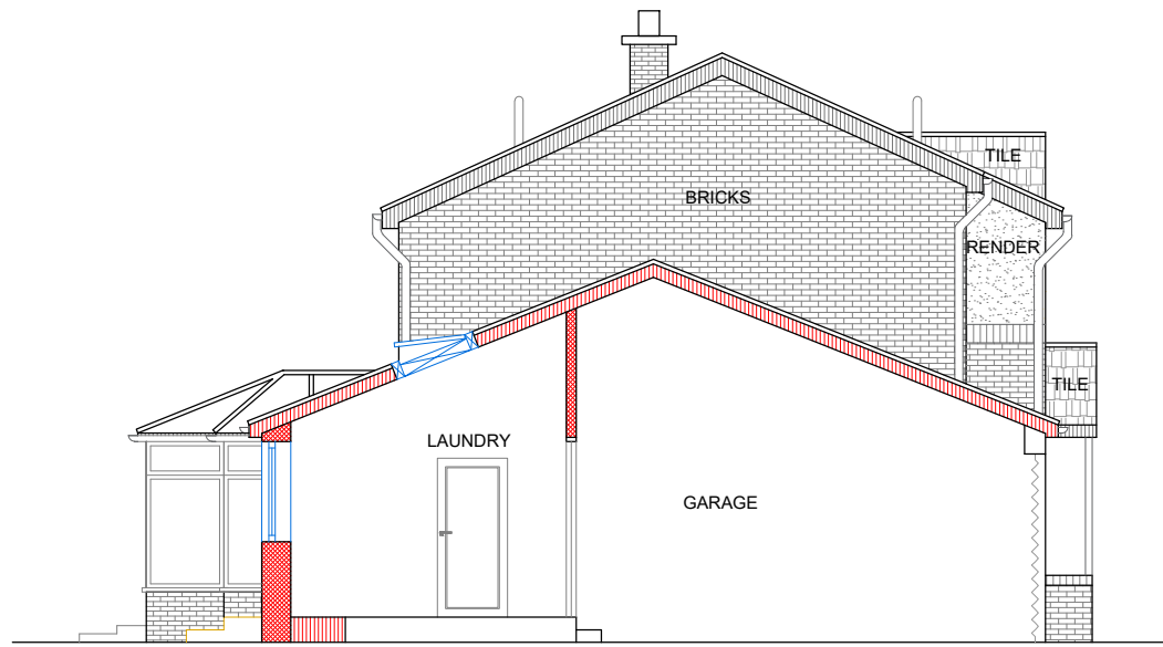
PROPOSED SECTION
