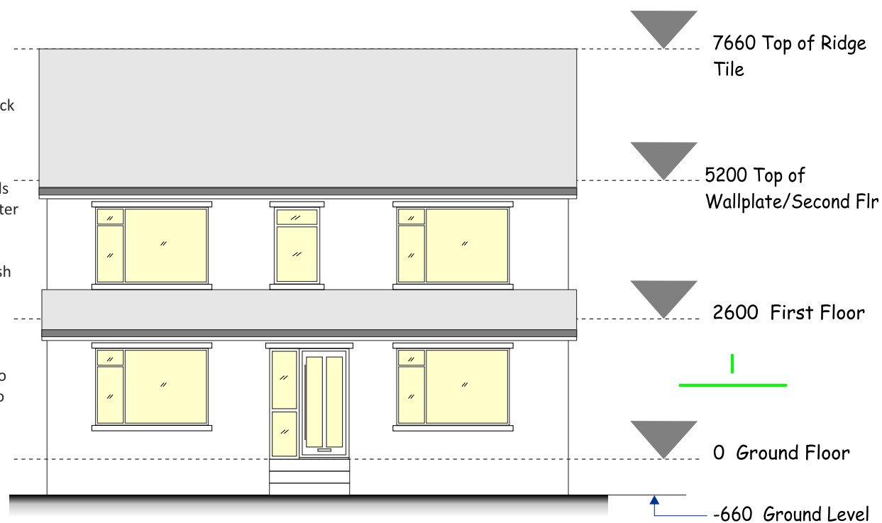
Proposed Front Elevation Scale 1:100 (Ref: HD45DB47v4)
