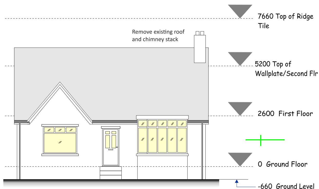
Existing Front Elevation Scale 1:100 (Ref: HD45DB47v4)
