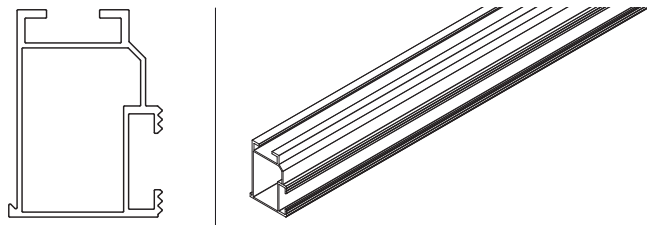
VS+ Rail connector 50 x 37
