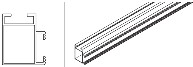
VS+ Mounting rail 50 x 37
